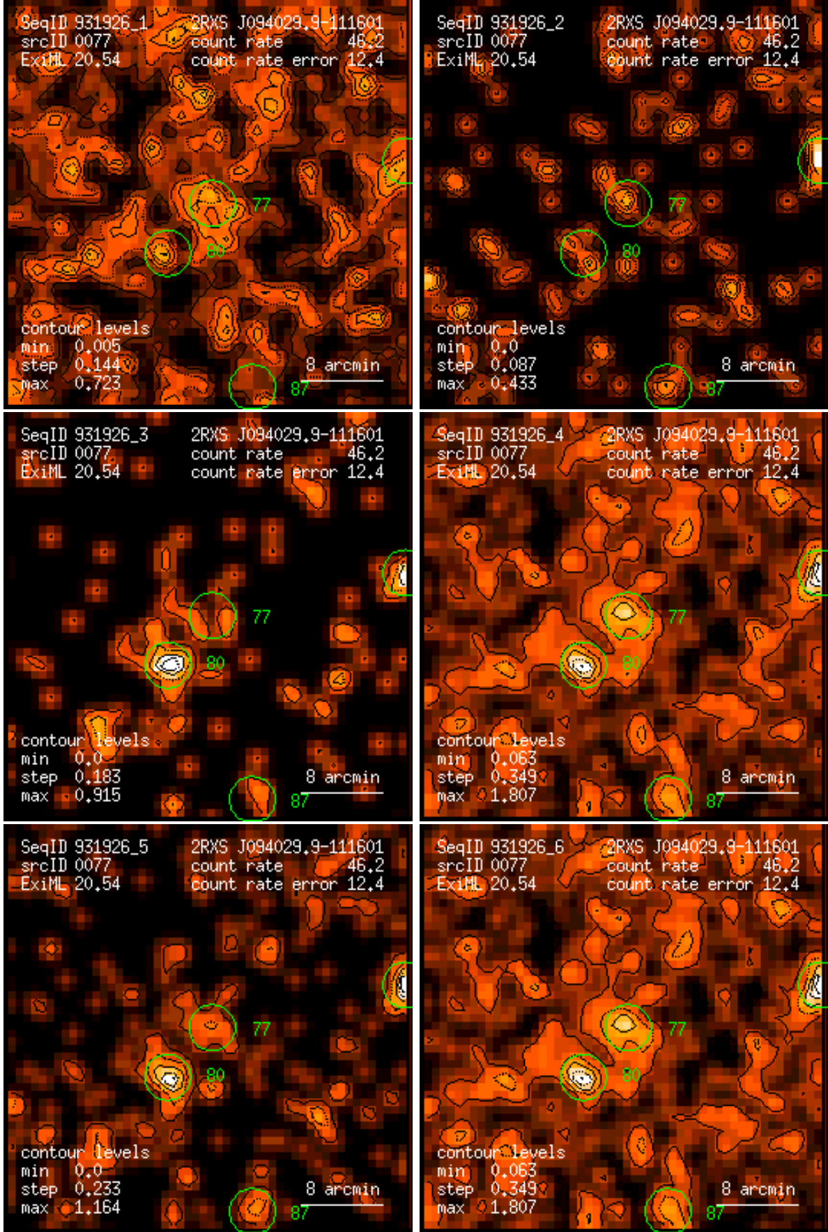
Figure 77: RASS 931926: detection 0077: band rate images, Gaussian filter: (1) PSPC channels 11 – 41, (2) 52 – 90, (3) 91 – 201, (4) 11 – 235, (5) 52 – 201, (6) 11 – 201. Broad band rates in counts/ks. Band rate contour levels in counts/ks/arcmin 2 .
