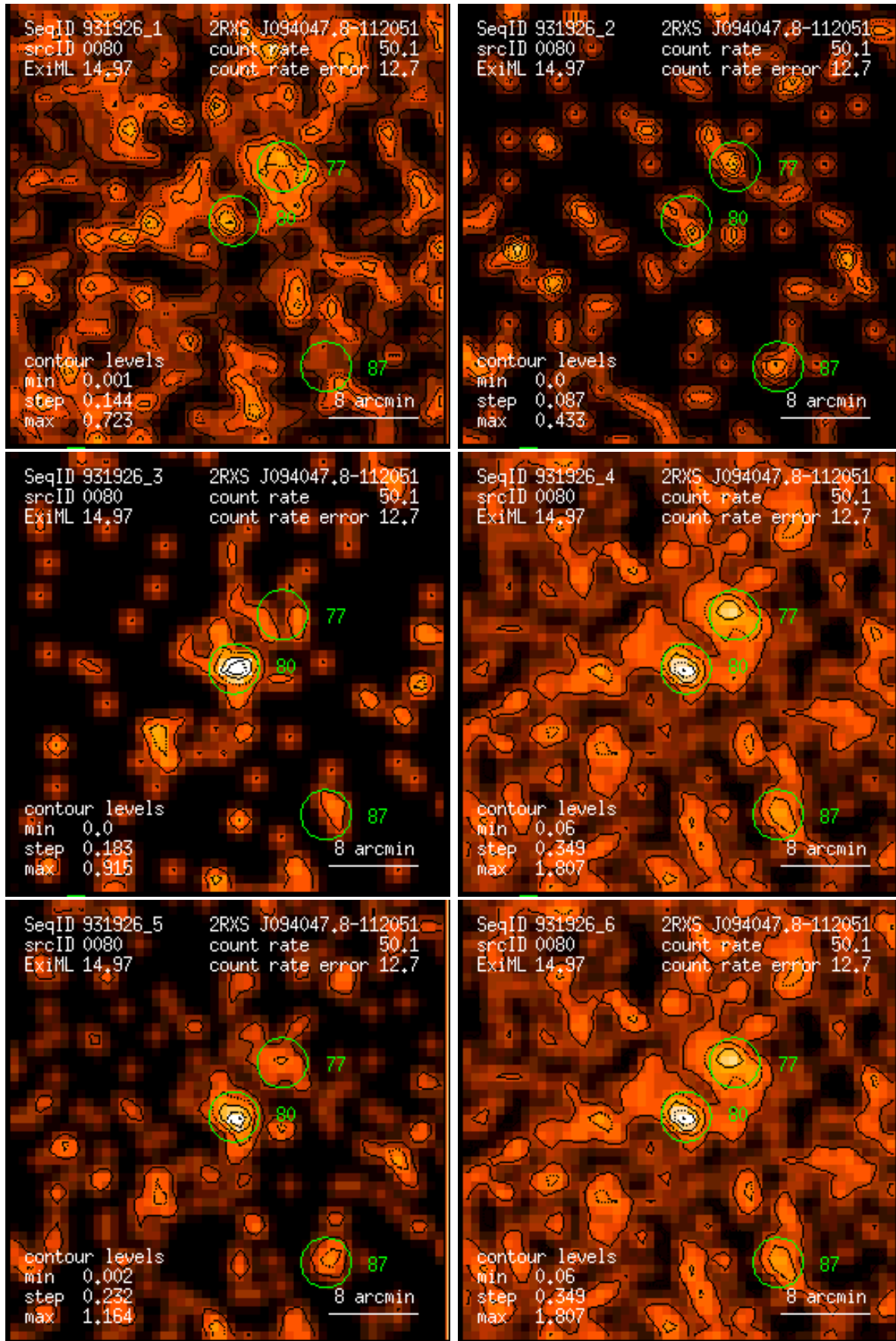
Figure 80: RASS 931926: detection 0080: band rate images, Gaussian filter: (1) PSPC channels 11 – 41, (2) 52 – 90, (3) 91 – 201, (4) 11 – 235, (5) 52 – 201, (6) 11 – 201. Broad band rates in counts/ks. Band rate contour levels in counts/ks/arcmin 2 .
