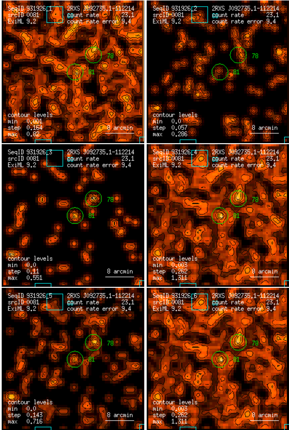
Figure 81: RASS 931926: detection 0081: band rate images, Gaussian filter: (1) PSPC channels 11 – 41, (2) 52 – 90, (3) 91 – 201, (4) 11 – 235, (5) 52 – 201, (6) 11 – 201. Broad band rates in counts/ks. Band rate contour levels in counts/ks/arcmin 2 .
