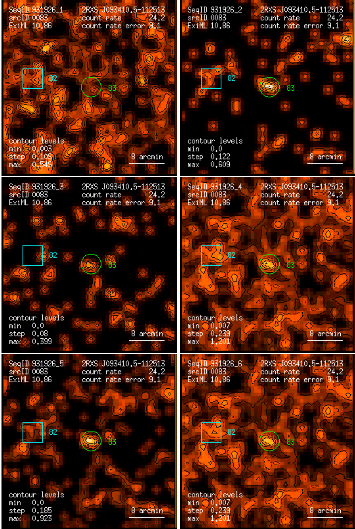
Figure 83: RASS 931926: detection 0083: band rate images, Gaussian filter: (1) PSPC channels 11 – 41, (2) 52 – 90, (3) 91 – 201, (4) 11 – 235, (5) 52 – 201, (6) 11 – 201. Broad band rates in counts/ks. Band rate contour levels in counts/ks/arcmin 2 .
