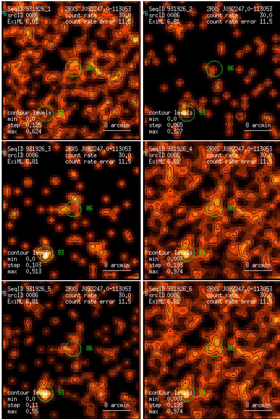
Figure 86: RASS 931926: detection 0086: band rate images, Gaussian filter: (1) PSPC channels 11 – 41, (2) 52 – 90, (3) 91 – 201, (4) 11 – 235, (5) 52 – 201, (6) 11 – 201. Broad band rates in counts/ks. Band rate contour levels in counts/ks/arcmin 2 .
