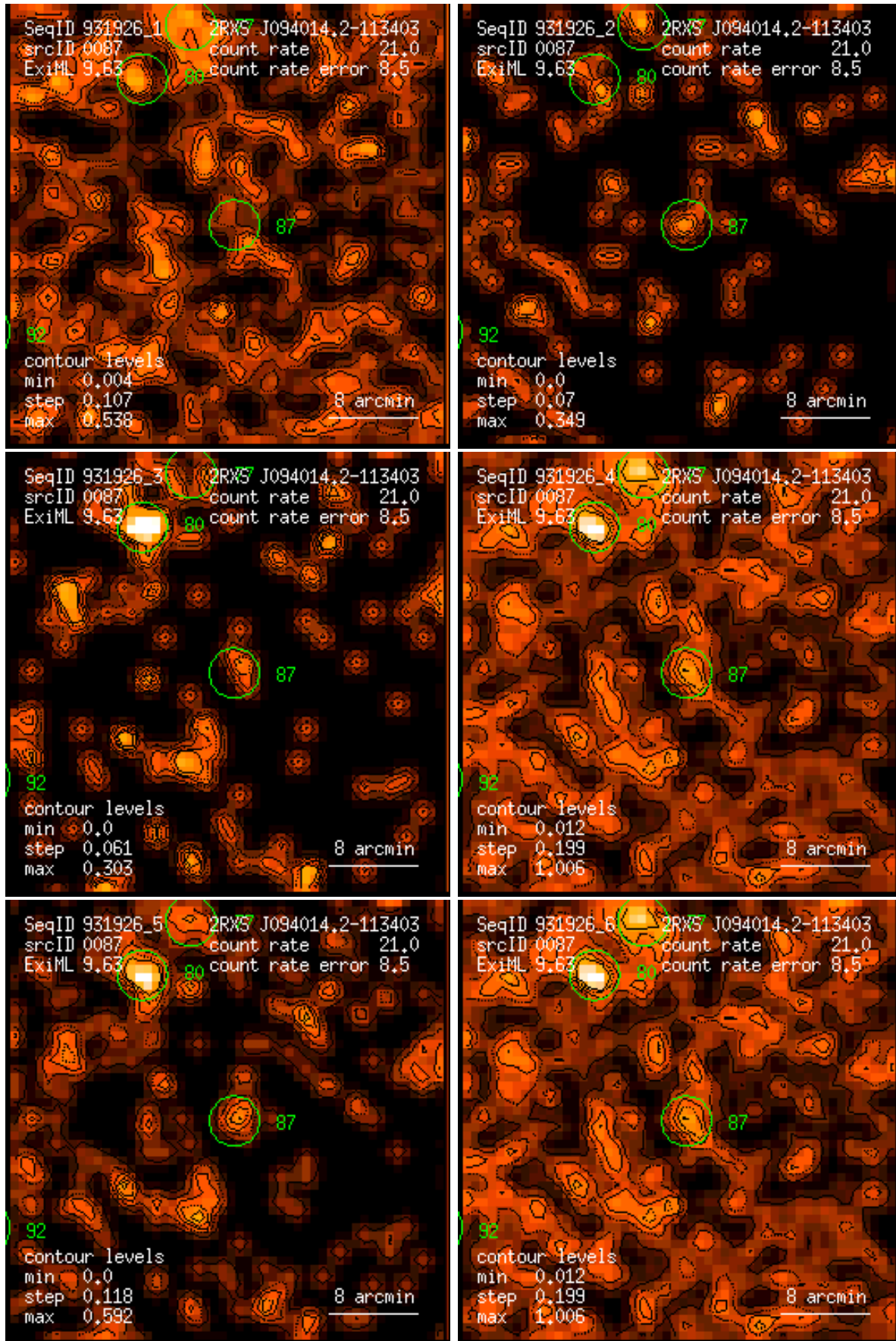
Figure 87: RASS 931926: detection 0087: band rate images, Gaussian filter: (1) PSPC channels 11 – 41, (2) 52 – 90, (3) 91 – 201, (4) 11 – 235, (5) 52 – 201, (6) 11 – 201. Broad band rates in counts/ks. Band rate contour levels in counts/ks/arcmin 2 .
