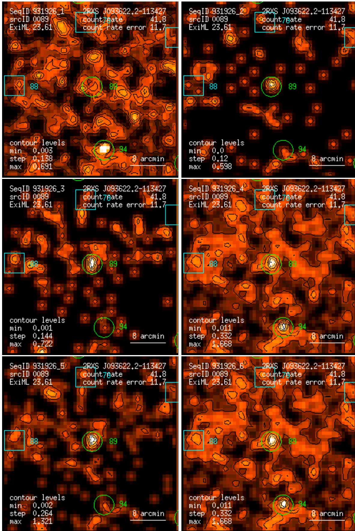
Figure 89: RASS 931926: detection 0089: band rate images, Gaussian filter: (1) PSPC channels 11 – 41, (2) 52 – 90, (3) 91 – 201, (4) 11 – 235, (5) 52 – 201, (6) 11 – 201. Broad band rates in counts/ks. Band rate contour levels in counts/ks/arcmin 2 .
