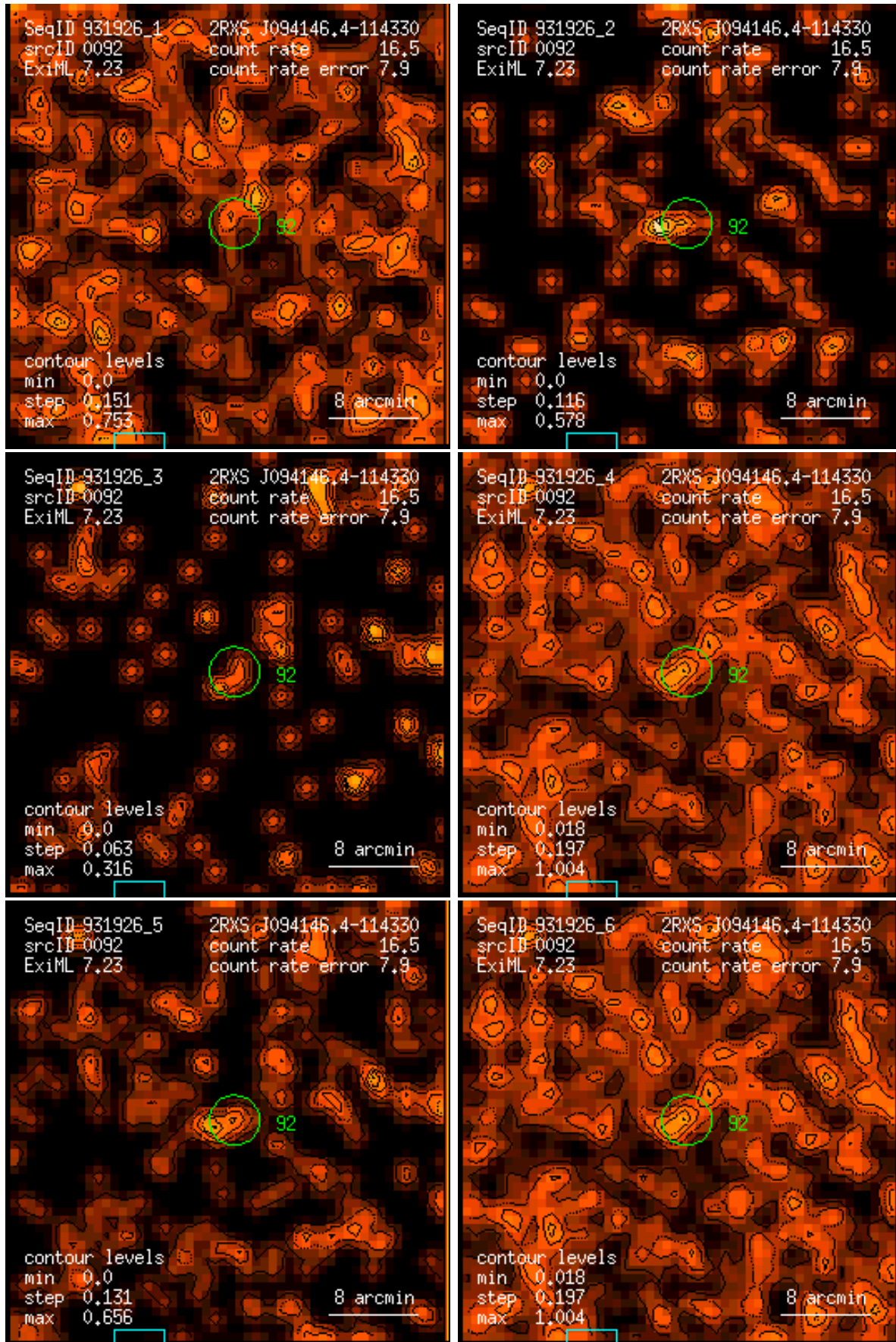
Figure 92: RASS 931926: detection 0092: band rate images, Gaussian filter: (1) PSPC channels 11 – 41, (2) 52 – 90, (3) 91 – 201, (4) 11 – 235, (5) 52 – 201, (6) 11 – 201. Broad band rates in counts/ks. Band rate contour levels in counts/ks/arcmin 2 .
