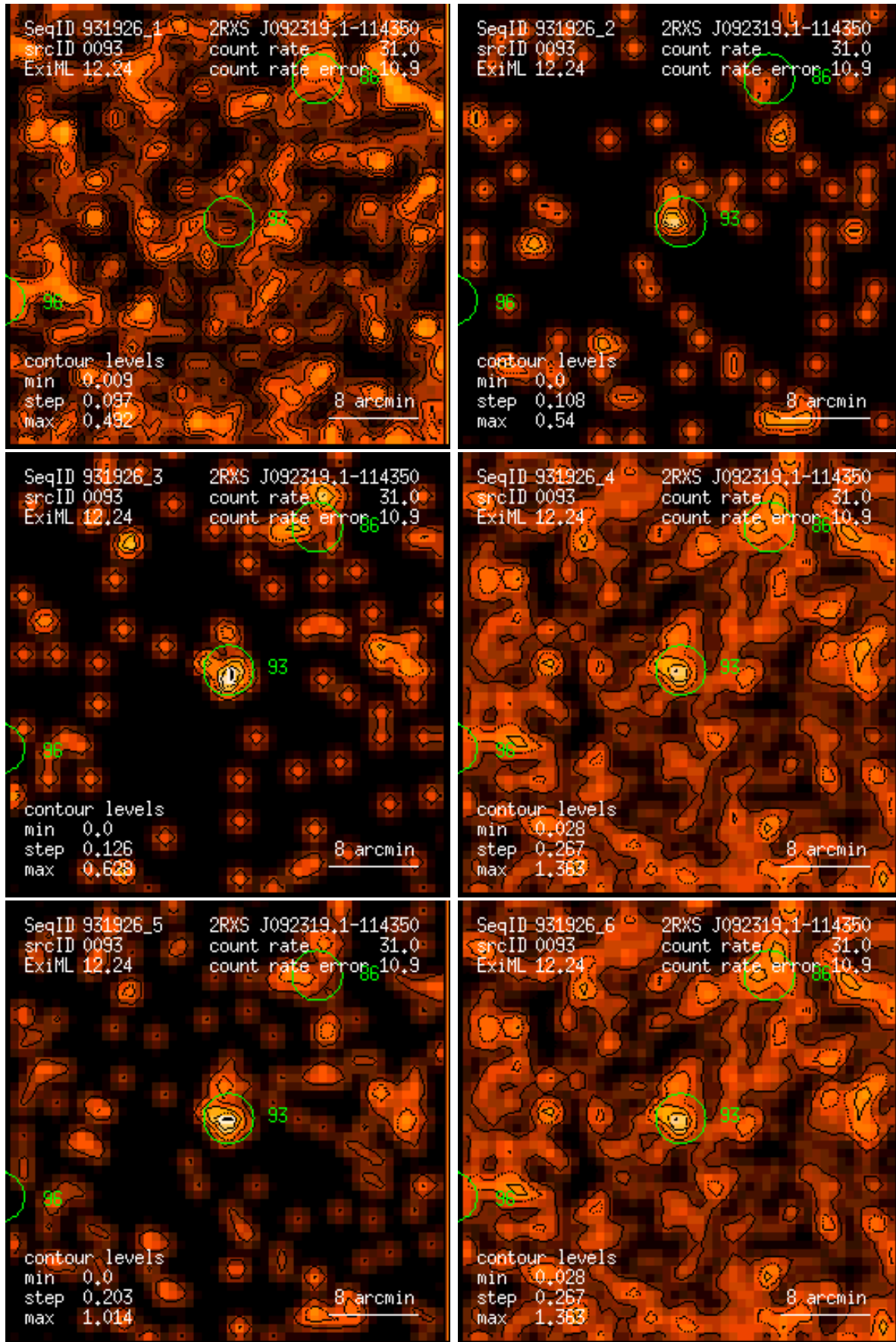
Figure 93: RASS 931926: detection 0093: band rate images, Gaussian filter: (1) PSPC channels 11 – 41, (2) 52 – 90, (3) 91 – 201, (4) 11 – 235, (5) 52 – 201, (6) 11 – 201. Broad band rates in counts/ks. Band rate contour levels in counts/ks/arcmin 2 .
