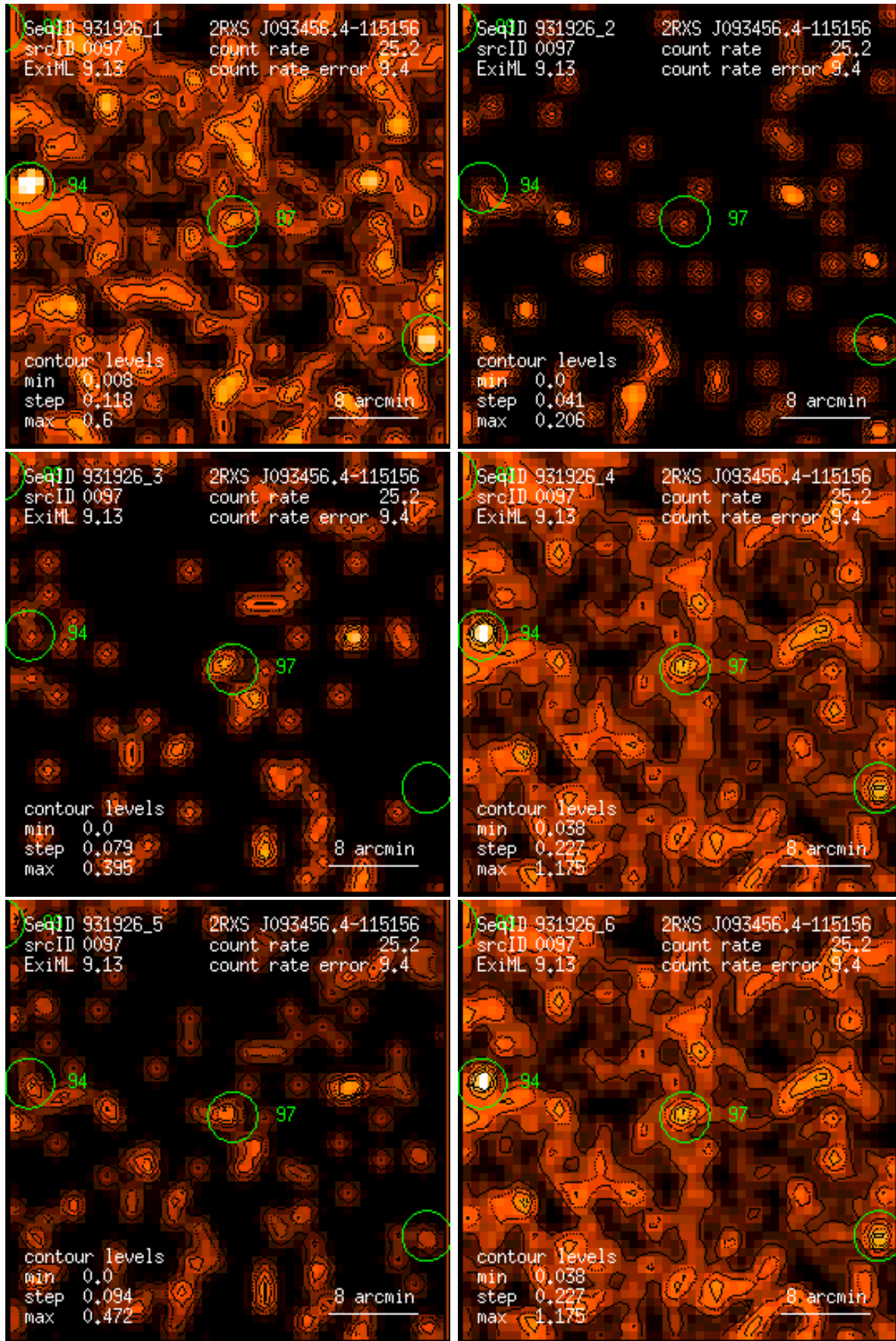
Figure 97: RASS 931926: detection 0097: band rate images, Gaussian filter: (1) PSPC channels 11 – 41, (2) 52 – 90, (3) 91 – 201, (4) 11 – 235, (5) 52 – 201, (6) 11 – 201. Broad band rates in counts/ks. Band rate contour levels in counts/ks/arcmin 2 .
