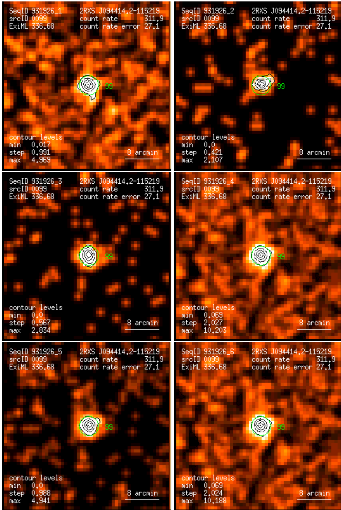
Figure 99: RASS 931926: detection 0099: band rate images, Gaussian filter: (1) PSPC channels 11 – 41, (2) 52 – 90, (3) 91 – 201, (4) 11 – 235, (5) 52 – 201, (6) 11 – 201. Broad band rates in counts/ks. Band rate contour levels in counts/ks/arcmin 2 .
