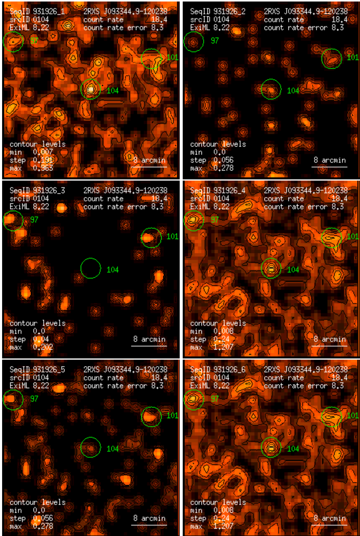
Figure 104: RASS 931926: detection 0104: band rate images, Gaussian filter: (1) PSPC channels 11 – 41, (2) 52 – 90, (3) 91 – 201, (4) 11 – 235, (5) 52 – 201, (6) 11 – 201. Broad band rates in counts/ks. Band rate contour levels in counts/ks/arcmin 2 .
