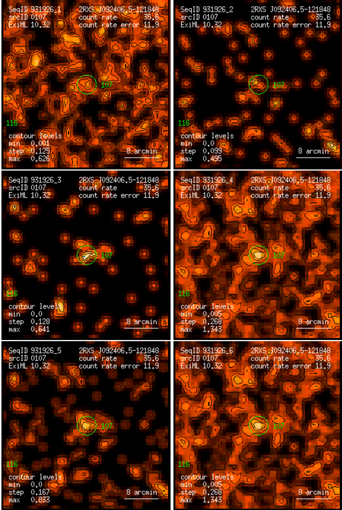
Figure 107: RASS 931926: detection 0107: band rate images, Gaussian filter: (1) PSPC channels 11 – 41, (2) 52 – 90, (3) 91 – 201, (4) 11 – 235, (5) 52 – 201, (6) 11 – 201. Broad band rates in counts/ks. Band rate contour levels in counts/ks/arcmin 2 .
