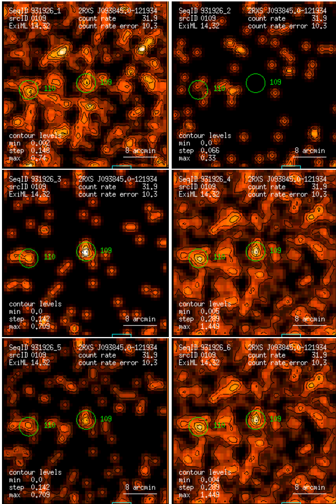
Figure 109: RASS 931926: detection 0109: band rate images, Gaussian filter: (1) PSPC channels 11 – 41, (2) 52 – 90, (3) 91 – 201, (4) 11 – 235, (5) 52 – 201, (6) 11 – 201. Broad band rates in counts/ks. Band rate contour levels in counts/ks/arcmin 2 .
