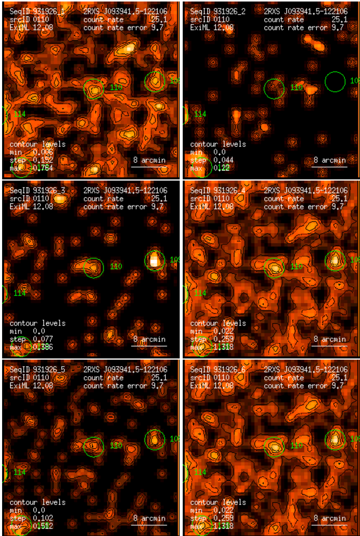
Figure 110: RASS 931926: detection 0110: band rate images, Gaussian filter: (1) PSPC channels 11 – 41, (2) 52 – 90, (3) 91 – 201, (4) 11 – 235, (5) 52 – 201, (6) 11 – 201. Broad band rates in counts/ks. Band rate contour levels in counts/ks/arcmin 2 .
