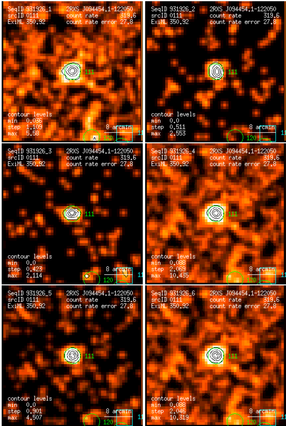
Figure 111: RASS 931926: detection 0111: band rate images, Gaussian filter: (1) PSPC channels 11 – 41, (2) 52 – 90, (3) 91 – 201, (4) 11 – 235, (5) 52 – 201, (6) 11 – 201. Broad band rates in counts/ks. Band rate contour levels in counts/ks/arcmin 2 .
