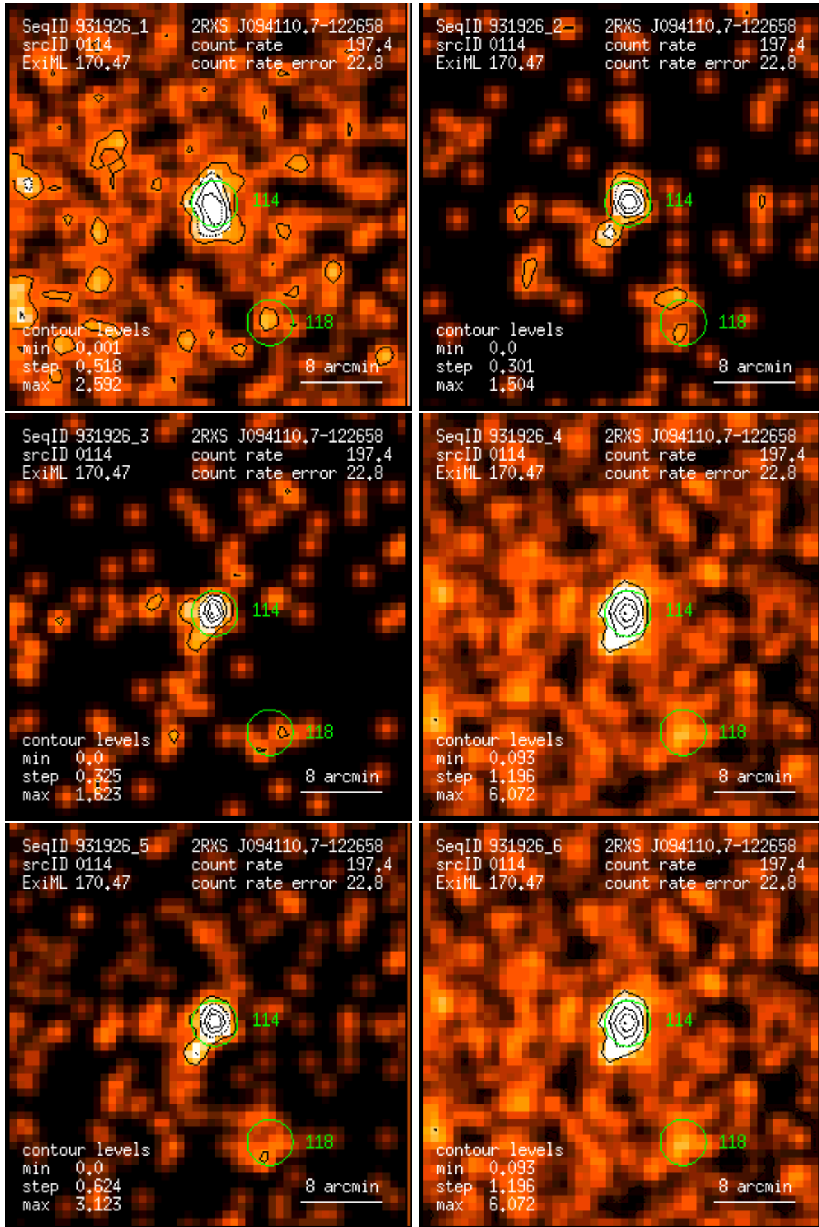
Figure 114: RASS 931926: detection 0114: band rate images, Gaussian filter: (1) PSPC channels 11 – 41, (2) 52 – 90, (3) 91 – 201, (4) 11 – 235, (5) 52 – 201, (6) 11 – 201. Broad band rates in counts/ks. Band rate contour levels in counts/ks/arcmin 2 .
