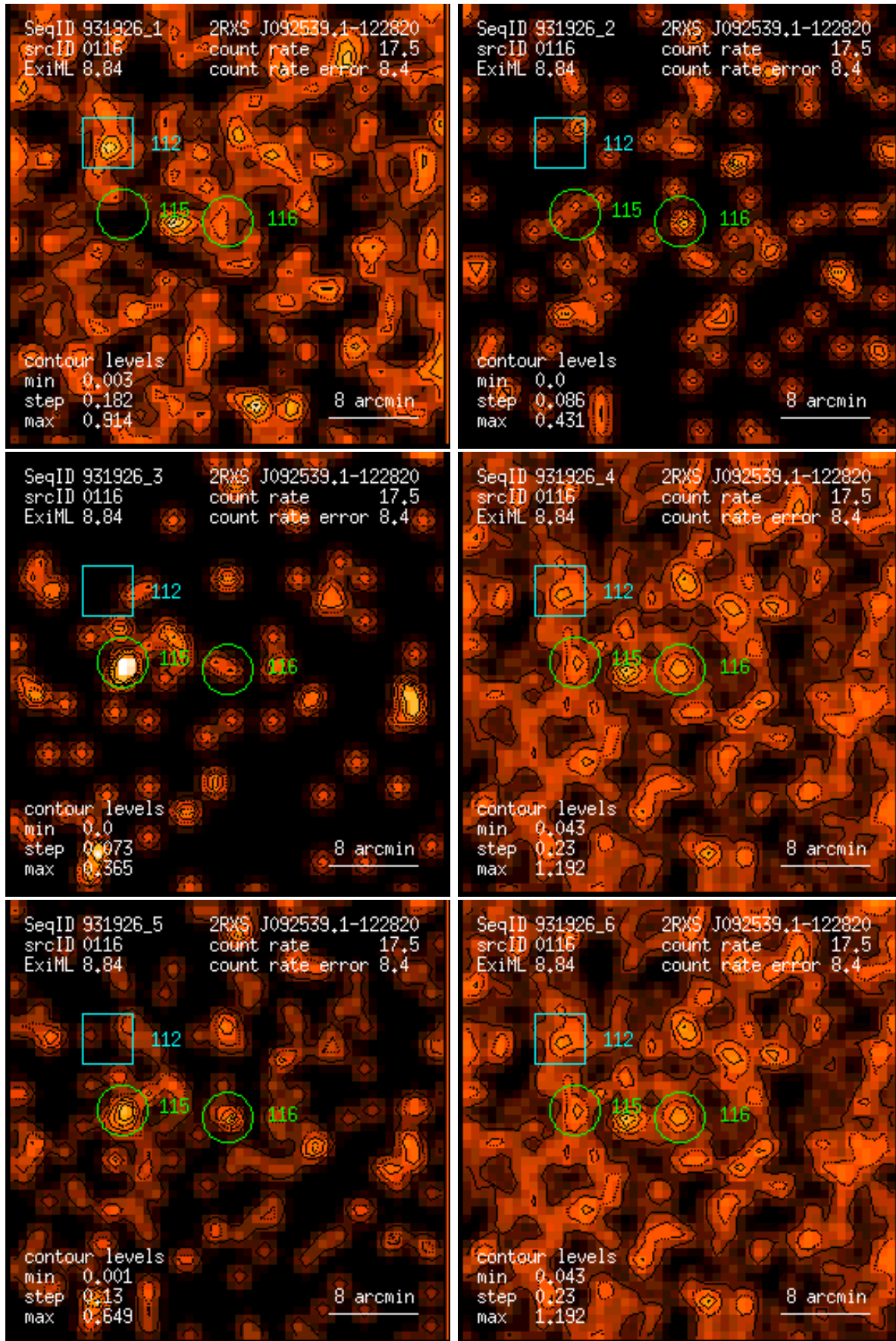
Figure 116: RASS 931926: detection 0116: band rate images, Gaussian filter: (1) PSPC channels 11 – 41, (2) 52 – 90, (3) 91 – 201, (4) 11 – 235, (5) 52 – 201, (6) 11 – 201. Broad band rates in counts/ks. Band rate contour levels in counts/ks/arcmin 2 .
