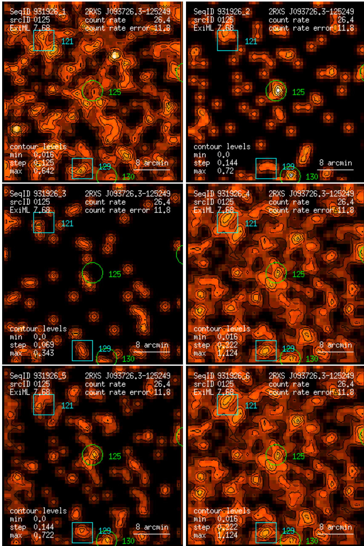
Figure 125: RASS 931926: detection 0125: band rate images, Gaussian filter: (1) PSPC channels 11 – 41, (2) 52 – 90, (3) 91 – 201, (4) 11 – 235, (5) 52 – 201, (6) 11 – 201. Broad band rates in counts/ks. Band rate contour levels in counts/ks/arcmin 2 .
