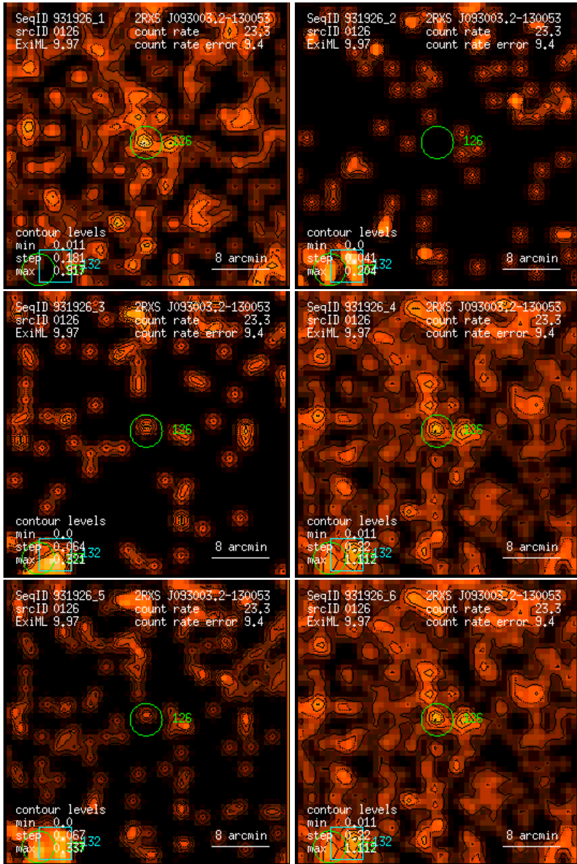
Figure 126: RASS 931926: detection 0126: band rate images, Gaussian filter: (1) PSPC channels 11 – 41, (2) 52 – 90, (3) 91 – 201, (4) 11 – 235, (5) 52 – 201, (6) 11 – 201. Broad band rates in counts/ks. Band rate contour levels in counts/ks/arcmin 2 .
