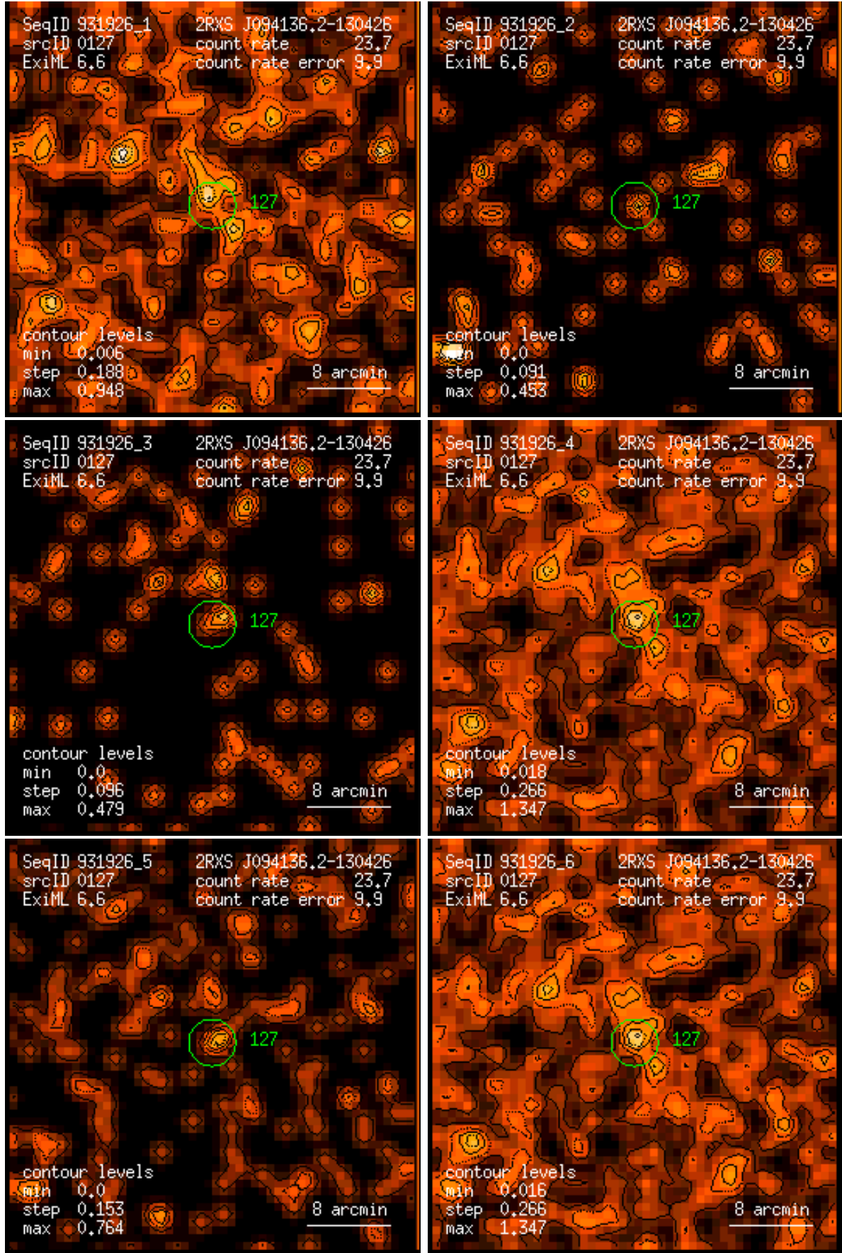
Figure 127: RASS 931926: detection 0127: band rate images, Gaussian filter: (1) PSPC channels 11 – 41, (2) 52 – 90, (3) 91 – 201, (4) 11 – 235, (5) 52 – 201, (6) 11 – 201. Broad band rates in counts/ks. Band rate contour levels in counts/ks/arcmin 2 .
