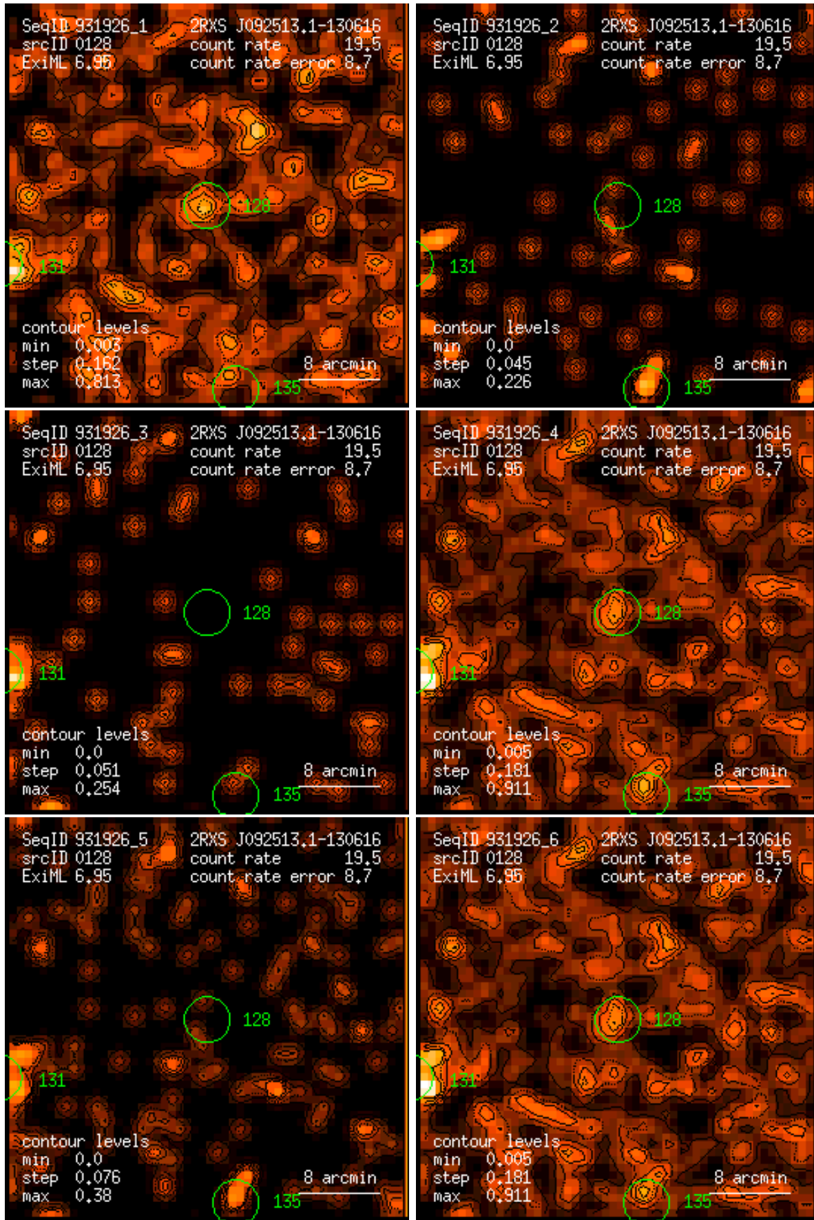
Figure 128: RASS 931926: detection 0128: band rate images, Gaussian filter: (1) PSPC channels 11 – 41, (2) 52 – 90, (3) 91 – 201, (4) 11 – 235, (5) 52 – 201, (6) 11 – 201. Broad band rates in counts/ks. Band rate contour levels in counts/ks/arcmin 2 .
