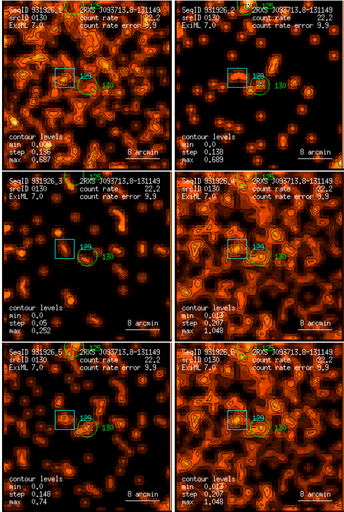
Figure 130: RASS 931926: detection 0130: band rate images, Gaussian filter: (1) PSPC channels 11 – 41, (2) 52 – 90, (3) 91 – 201, (4) 11 – 235, (5) 52 – 201, (6) 11 – 201. Broad band rates in counts/ks. Band rate contour levels in counts/ks/arcmin 2 .
