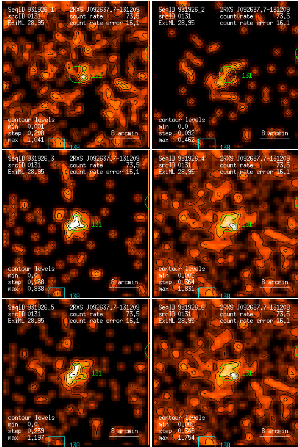
Figure 131: RASS 931926: detection 0131: band rate images, Gaussian filter: (1) PSPC channels 11 – 41, (2) 52 – 90, (3) 91 – 201, (4) 11 – 235, (5) 52 – 201, (6) 11 – 201. Broad band rates in counts/ks. Band rate contour levels in counts/ks/arcmin 2 .
