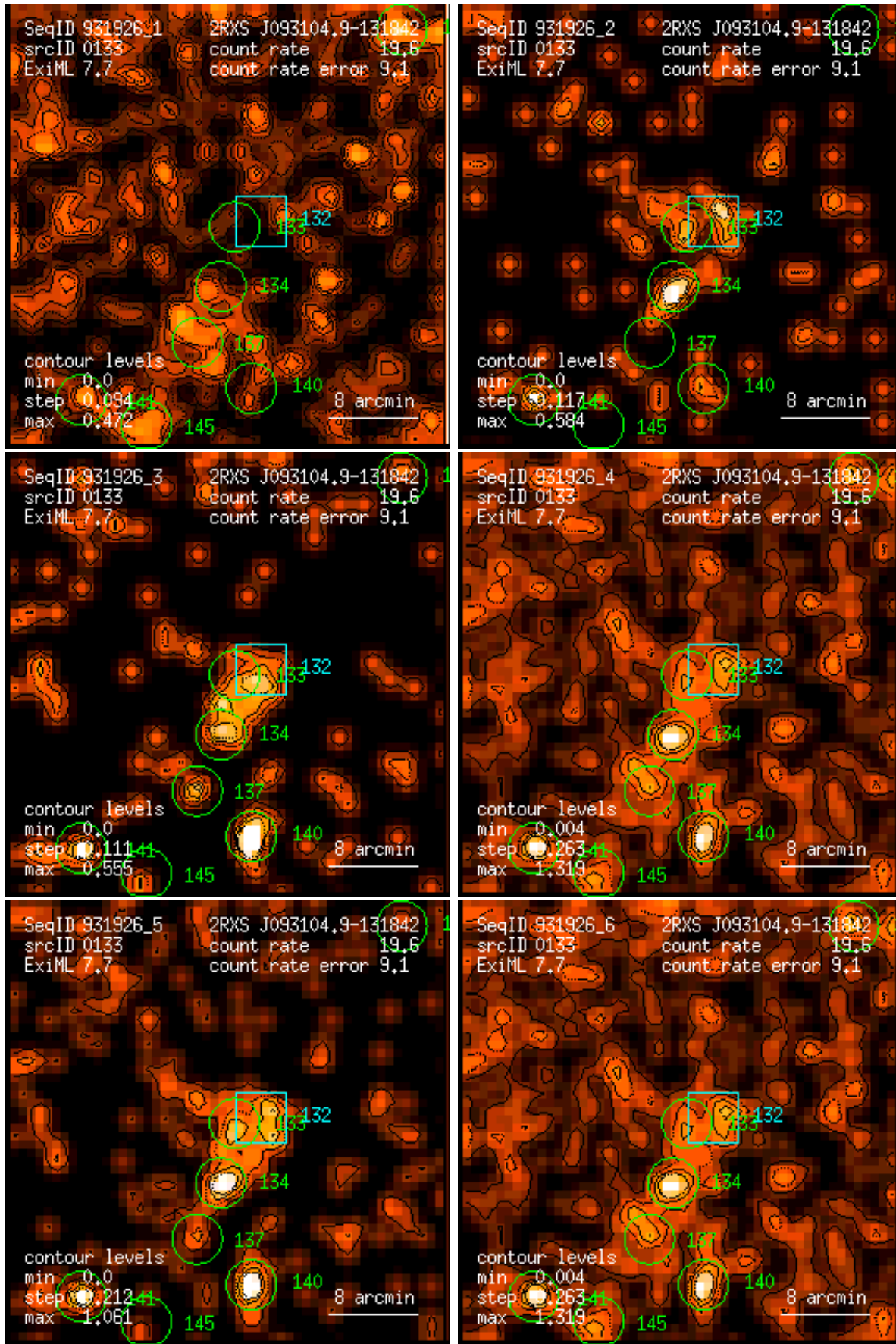
Figure 133: RASS 931926: detection 0133: band rate images, Gaussian filter: (1) PSPC channels 11 – 41, (2) 52 – 90, (3) 91 – 201, (4) 11 – 235, (5) 52 – 201, (6) 11 – 201. Broad band rates in counts/ks. Band rate contour levels in counts/ks/arcmin 2 .
