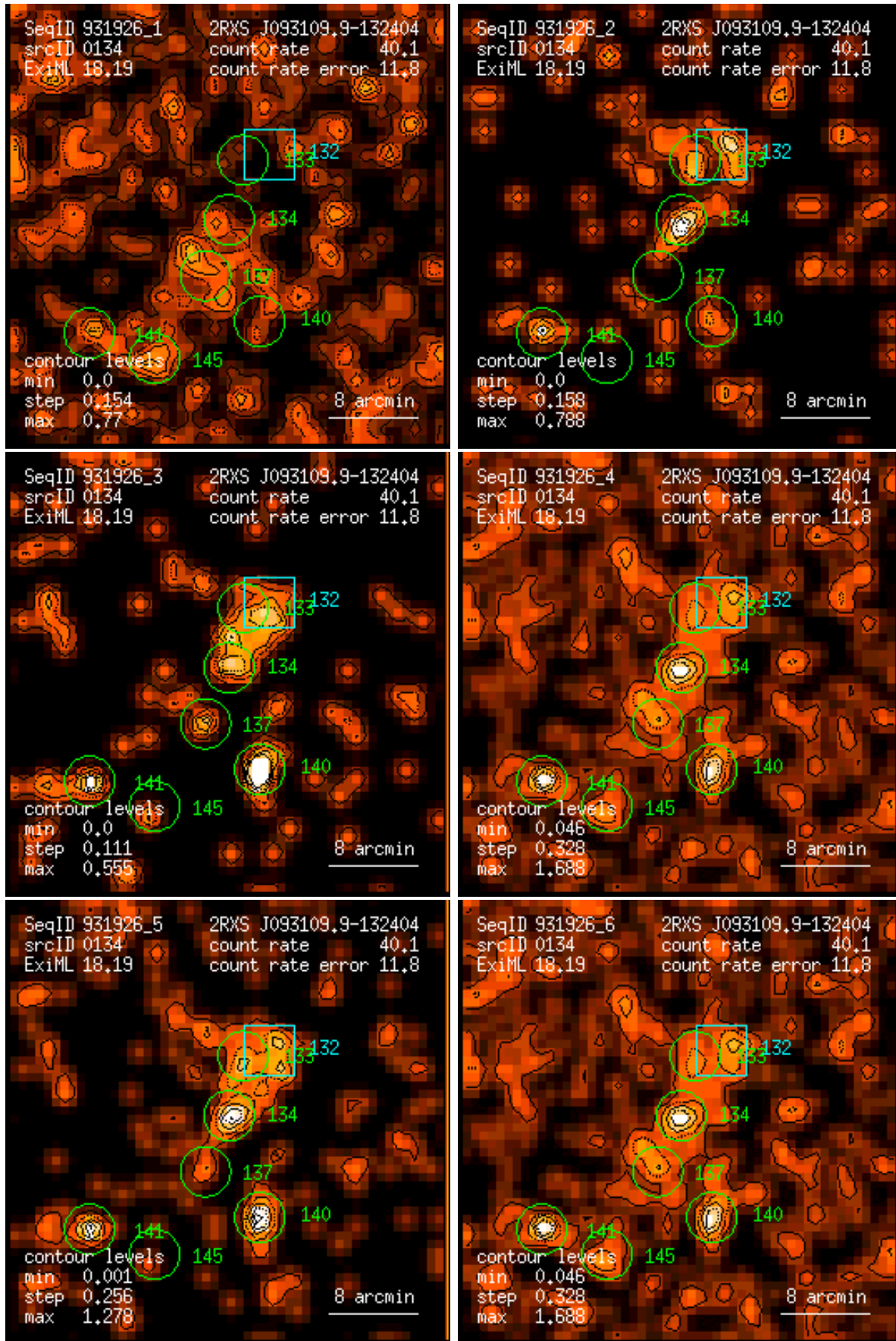
Figure 134: RASS 931926: detection 0134: band rate images, Gaussian filter: (1) PSPC channels 11 – 41, (2) 52 – 90, (3) 91 – 201, (4) 11 – 235, (5) 52 – 201, (6) 11 – 201. Broad band rates in counts/ks. Band rate contour levels in counts/ks/arcmin 2 .
