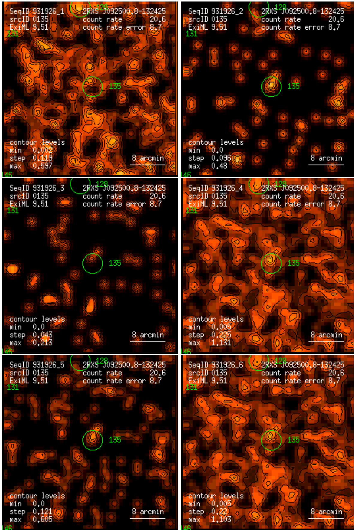
Figure 135: RASS 931926: detection 0135: band rate images, Gaussian filter: (1) PSPC channels 11 – 41, (2) 52 – 90, (3) 91 – 201, (4) 11 – 235, (5) 52 – 201, (6) 11 – 201. Broad band rates in counts/ks. Band rate contour levels in counts/ks/arcmin 2 .
