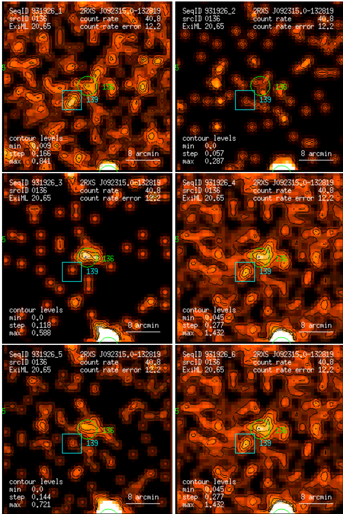
Figure 136: RASS 931926: detection 0136: band rate images, Gaussian filter: (1) PSPC channels 11 – 41, (2) 52 – 90, (3) 91 – 201, (4) 11 – 235, (5) 52 – 201, (6) 11 – 201. Broad band rates in counts/ks. Band rate contour levels in counts/ks/arcmin 2 .
