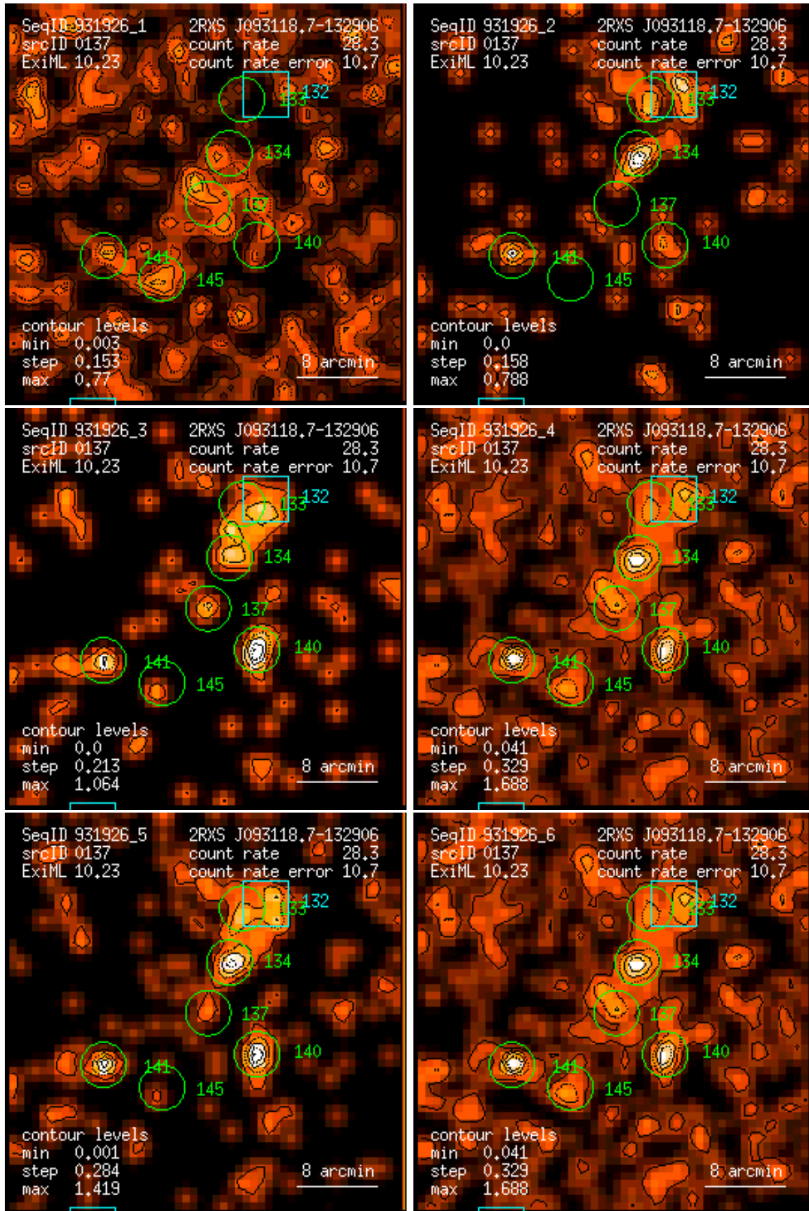
Figure 137: RASS 931926: detection 0137: band rate images, Gaussian filter: (1) PSPC channels 11 – 41, (2) 52 – 90, (3) 91 – 201, (4) 11 – 235, (5) 52 – 201, (6) 11 – 201. Broad band rates in counts/ks. Band rate contour levels in counts/ks/arcmin 2 .
