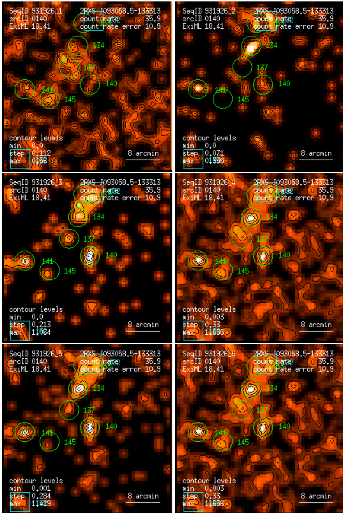
Figure 140: RASS 931926: detection 0140: band rate images, Gaussian filter: (1) PSPC channels 11 – 41, (2) 52 – 90, (3) 91 – 201, (4) 11 – 235, (5) 52 – 201, (6) 11 – 201. Broad band rates in counts/ks. Band rate contour levels in counts/ks/arcmin 2 .
