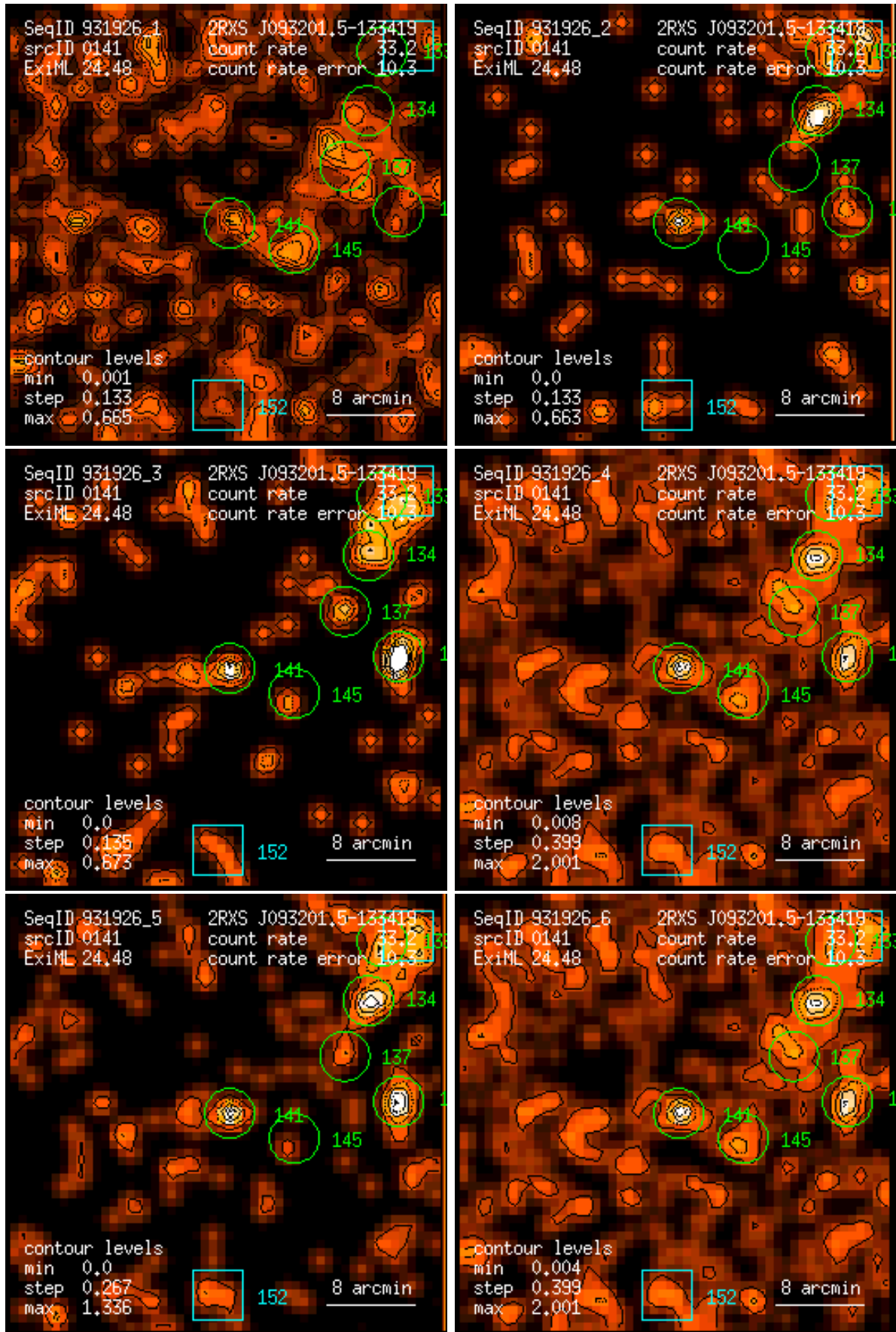
Figure 141: RASS 931926: detection 0141: band rate images, Gaussian filter: (1) PSPC channels 11 – 41, (2) 52 – 90, (3) 91 – 201, (4) 11 – 235, (5) 52 – 201, (6) 11 – 201. Broad band rates in counts/ks. Band rate contour levels in counts/ks/arcmin 2 .
