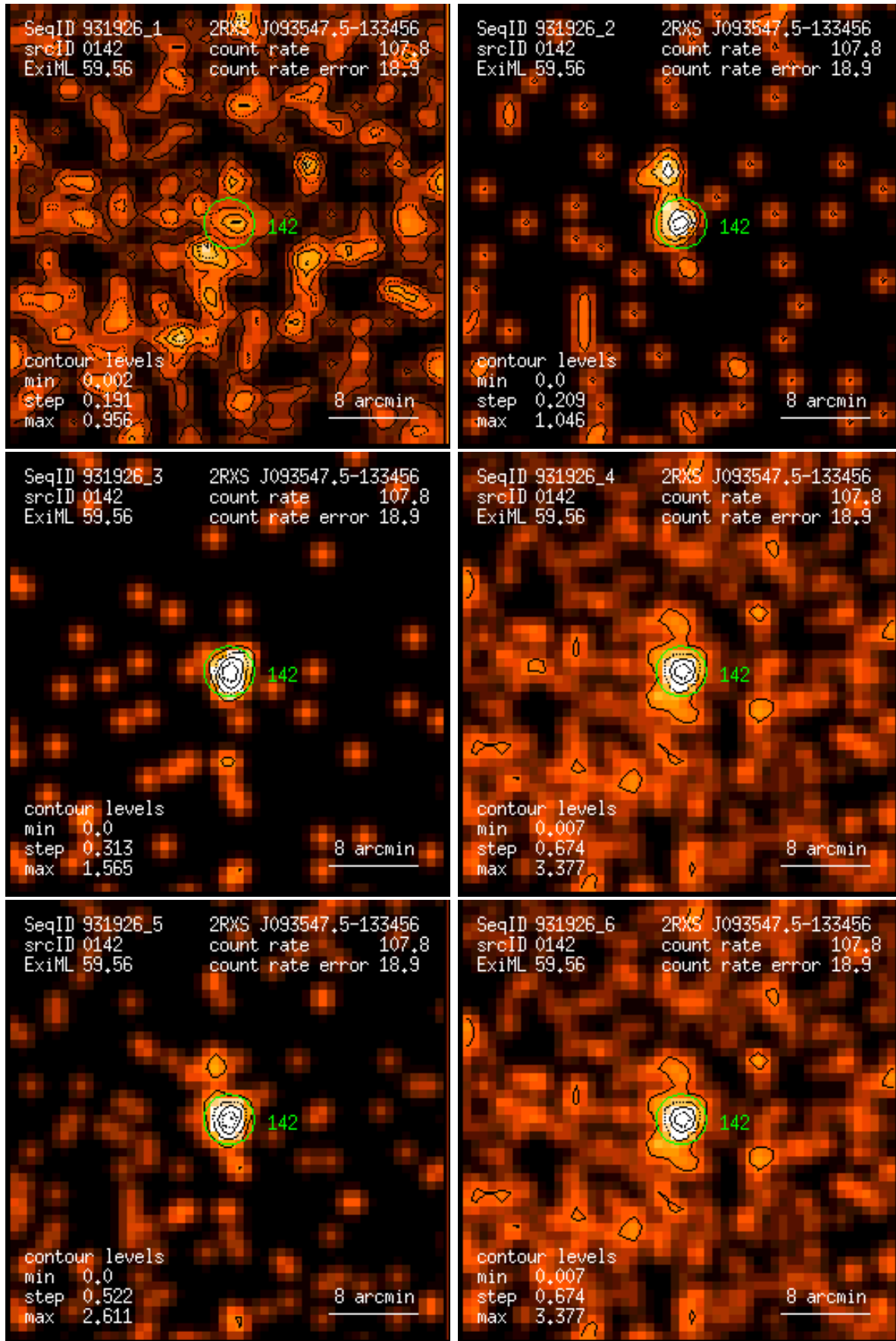
Figure 142: RASS 931926: detection 0142: band rate images, Gaussian filter: (1) PSPC channels 11 – 41, (2) 52 – 90, (3) 91 – 201, (4) 11 – 235, (5) 52 – 201, (6) 11 – 201. Broad band rates in counts/ks. Band rate contour levels in counts/ks/arcmin 2 .
