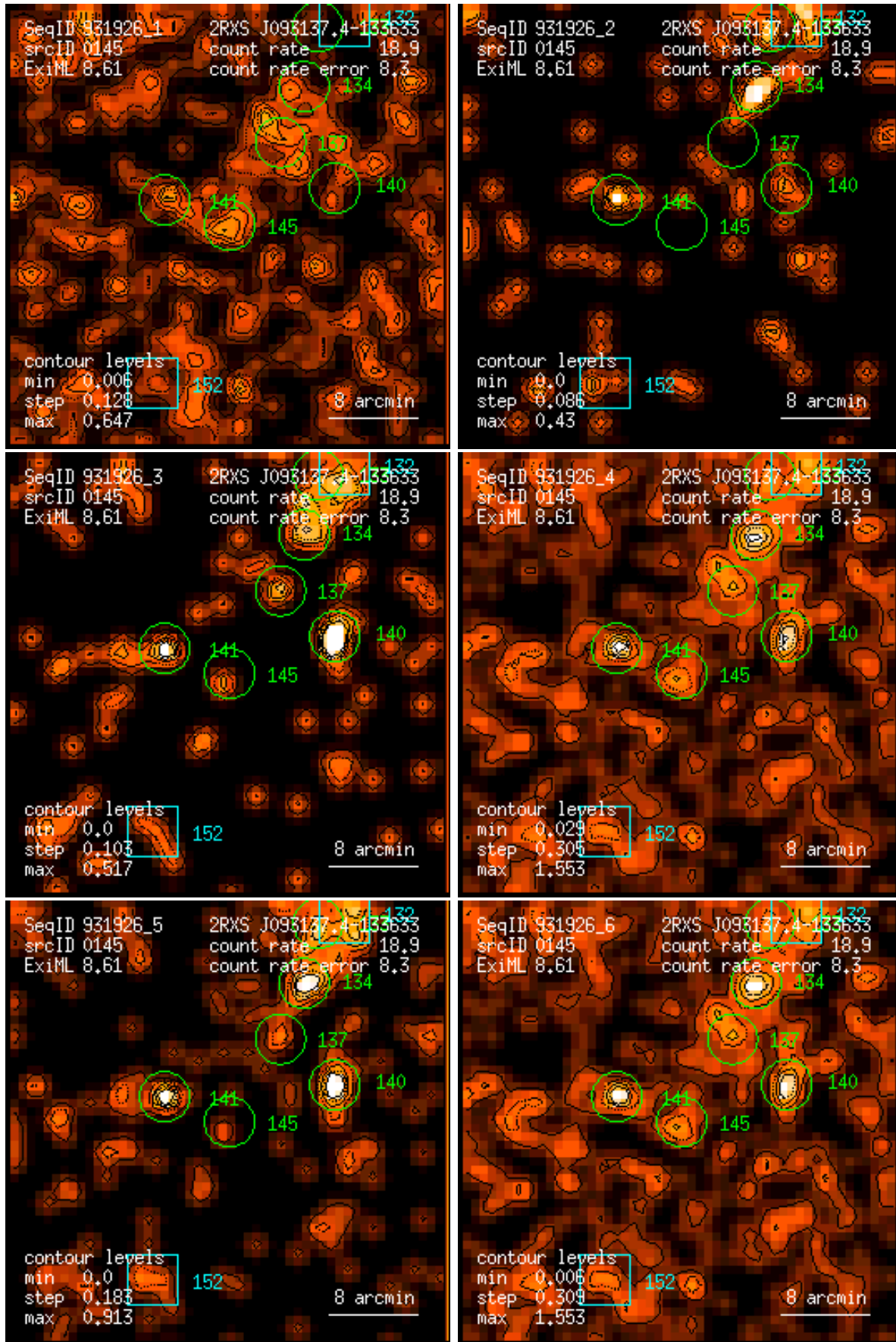
Figure 145: RASS 931926: detection 0145: band rate images, Gaussian filter: (1) PSPC channels 11 – 41, (2) 52 – 90, (3) 91 – 201, (4) 11 – 235, (5) 52 – 201, (6) 11 – 201. Broad band rates in counts/ks. Band rate contour levels in counts/ks/arcmin 2 .
