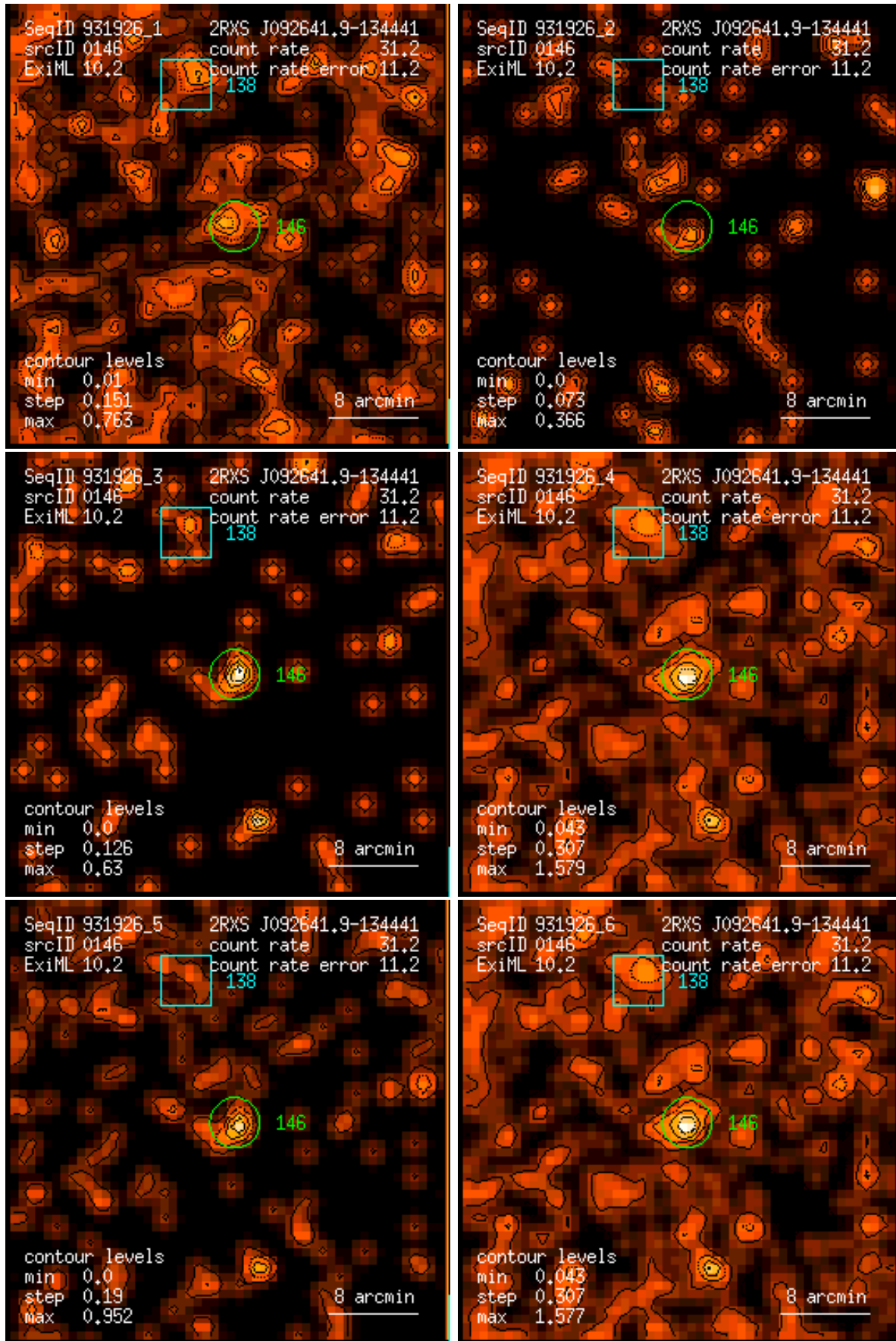
Figure 146: RASS 931926: detection 0146: band rate images, Gaussian filter: (1) PSPC channels 11 – 41, (2) 52 – 90, (3) 91 – 201, (4) 11 – 235, (5) 52 – 201, (6) 11 – 201. Broad band rates in counts/ks. Band rate contour levels in counts/ks/arcmin 2 .
