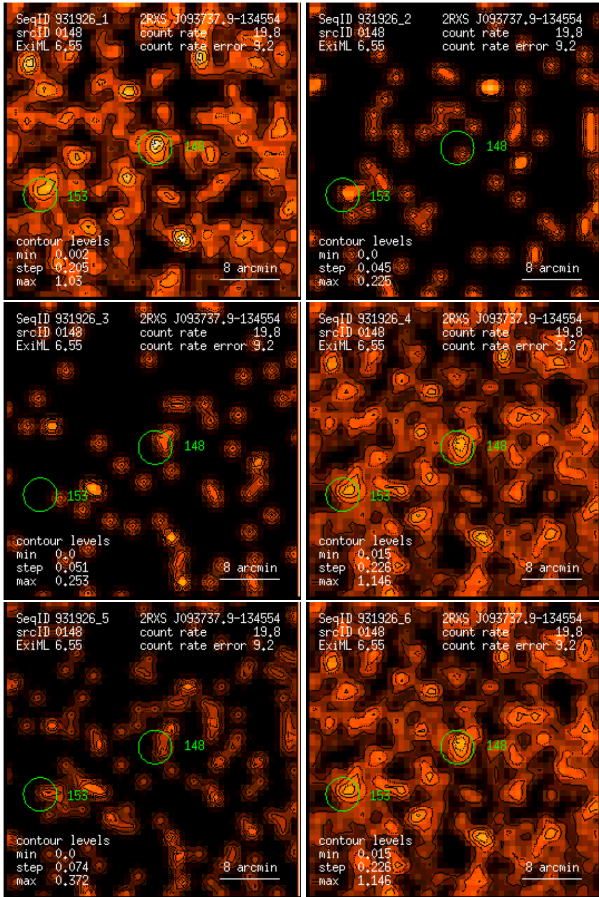
Figure 148: RASS 931926: detection 0148: band rate images, Gaussian filter: (1) PSPC channels 11 – 41, (2) 52 – 90, (3) 91 – 201, (4) 11 – 235, (5) 52 – 201, (6) 11 – 201. Broad band rates in counts/ks. Band rate contour levels in counts/ks/arcmin 2 .
