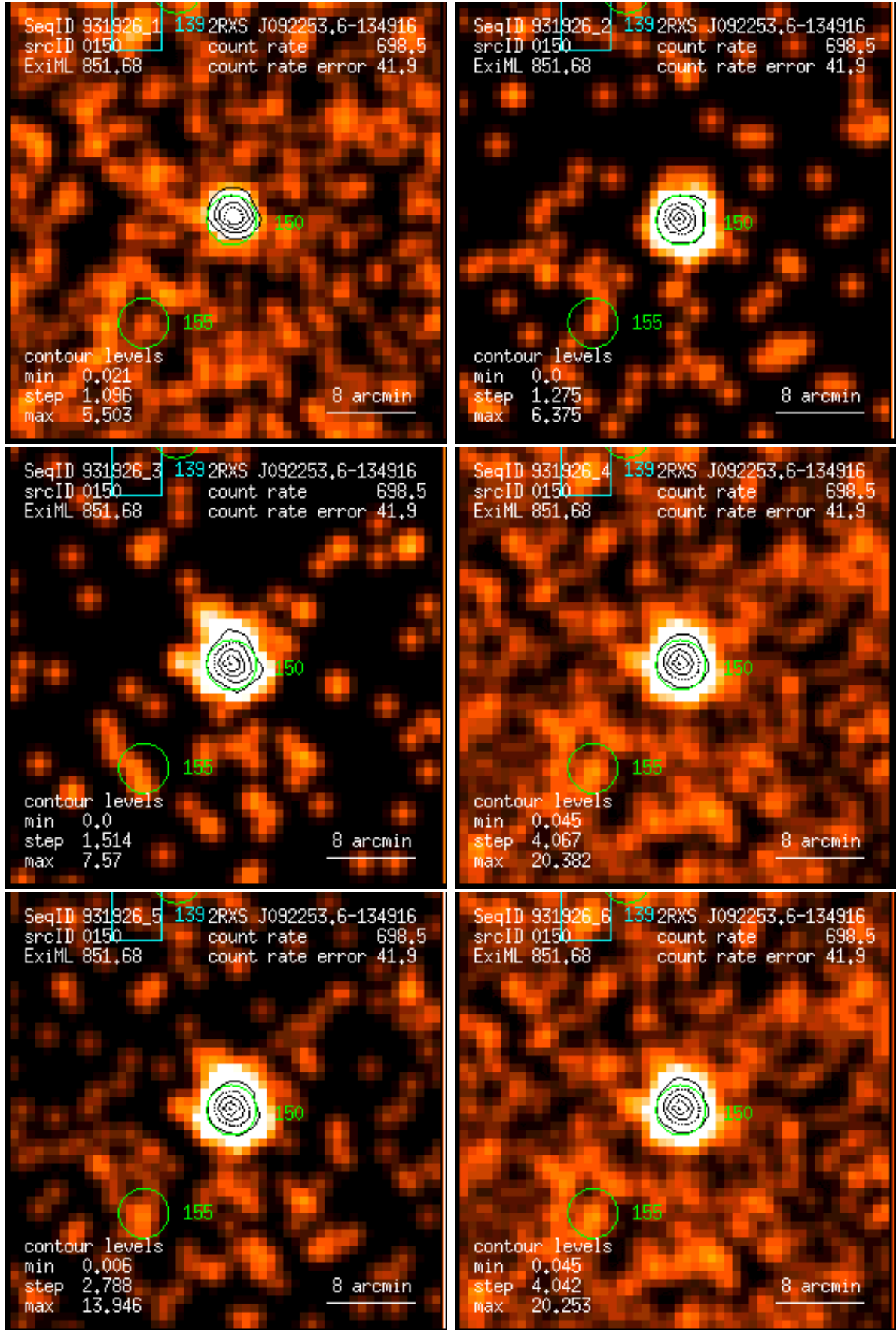
Figure 150: RASS 931926: detection 0150: band rate images, Gaussian filter: (1) PSPC channels 11 – 41, (2) 52 – 90, (3) 91 – 201, (4) 11 – 235, (5) 52 – 201, (6) 11 – 201. Broad band rates in counts/ks. Band rate contour levels in counts/ks/arcmin 2 .
