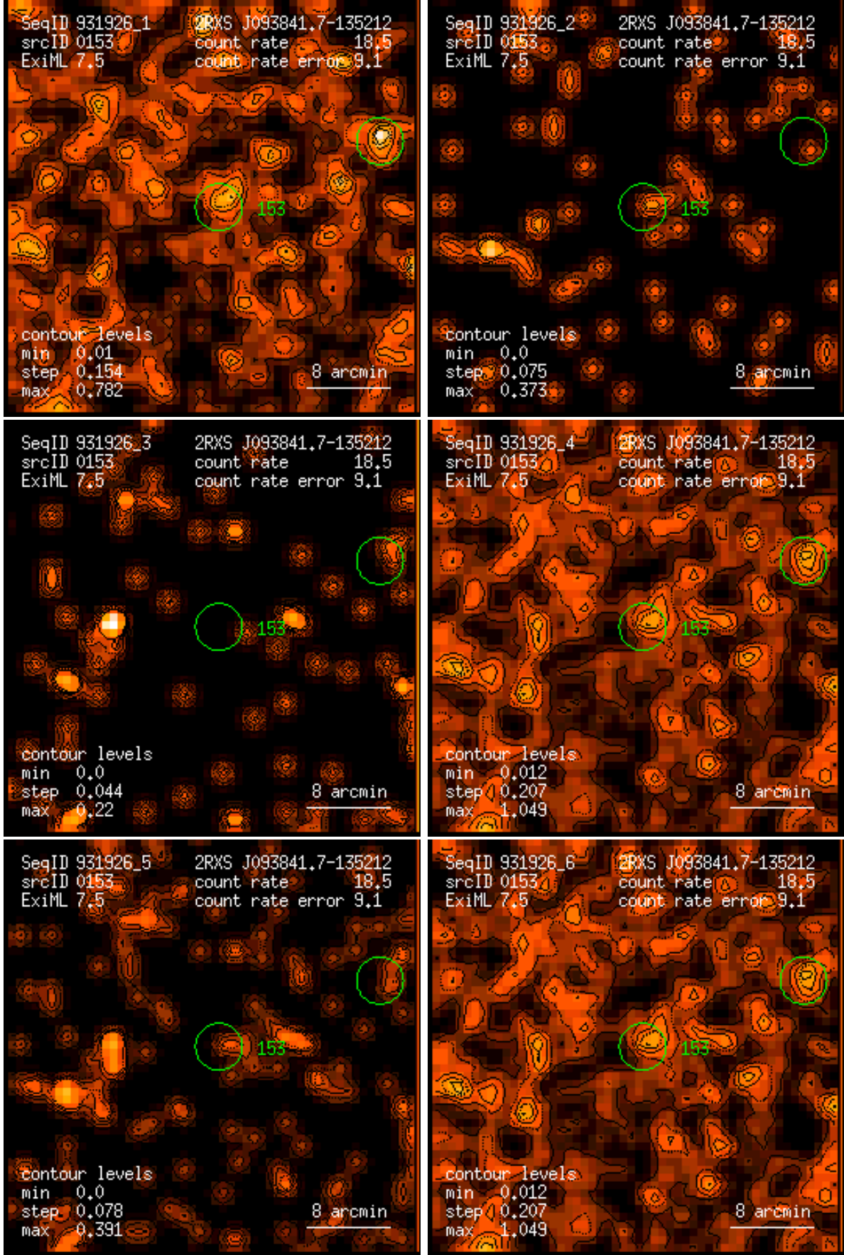
Figure 153: RASS 931926: detection 0153: band rate images, Gaussian filter: (1) PSPC channels 11 – 41, (2) 52 – 90, (3) 91 – 201, (4) 11 – 235, (5) 52 – 201, (6) 11 – 201. Broad band rates in counts/ks. Band rate contour levels in counts/ks/arcmin 2 .
