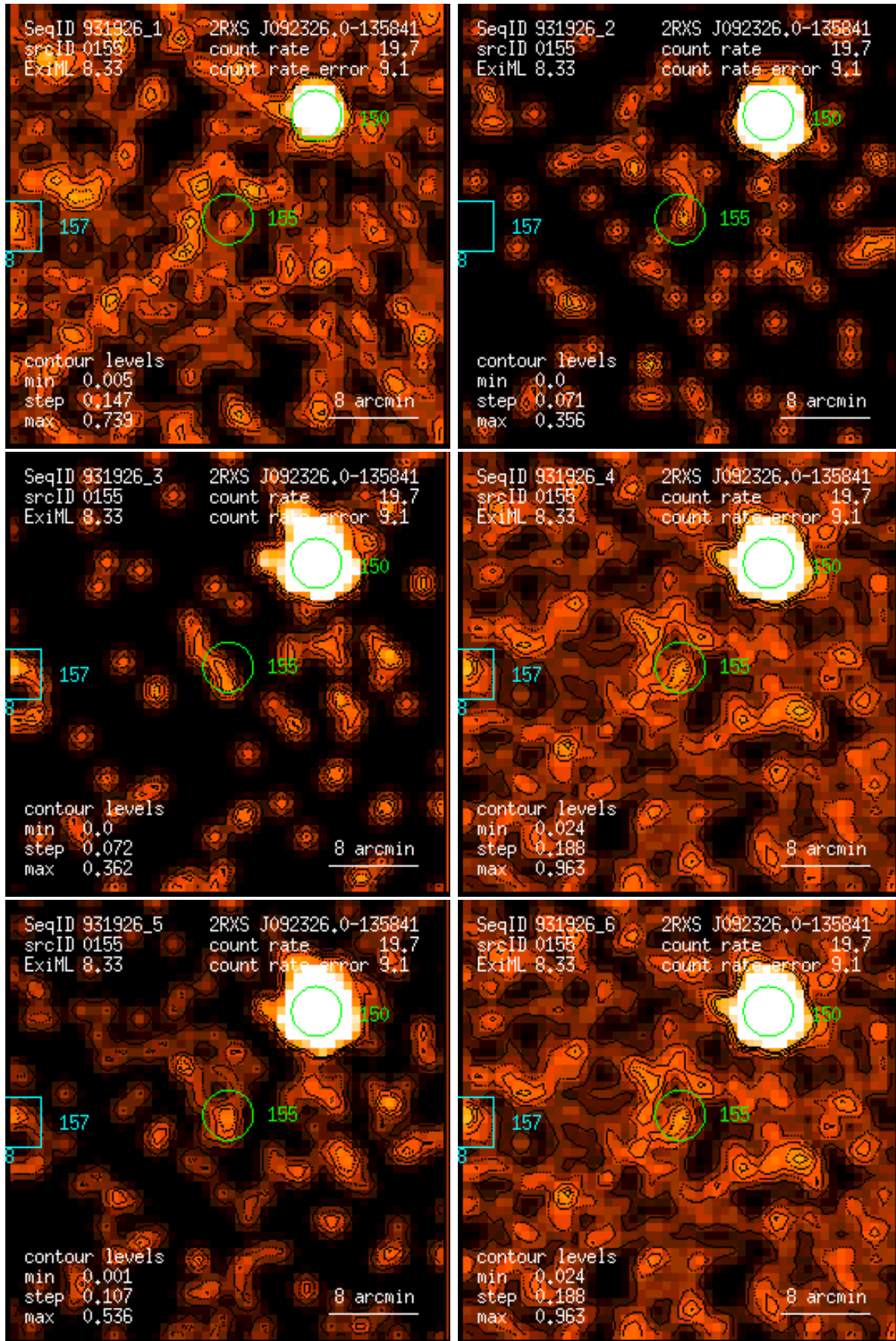
Figure 155: RASS 931926: detection 0155: band rate images, Gaussian filter: (1) PSPC channels 11 – 41, (2) 52 – 90, (3) 91 – 201, (4) 11 – 235, (5) 52 – 201, (6) 11 – 201. Broad band rates in counts/ks. Band rate contour levels in counts/ks/arcmin 2 .
