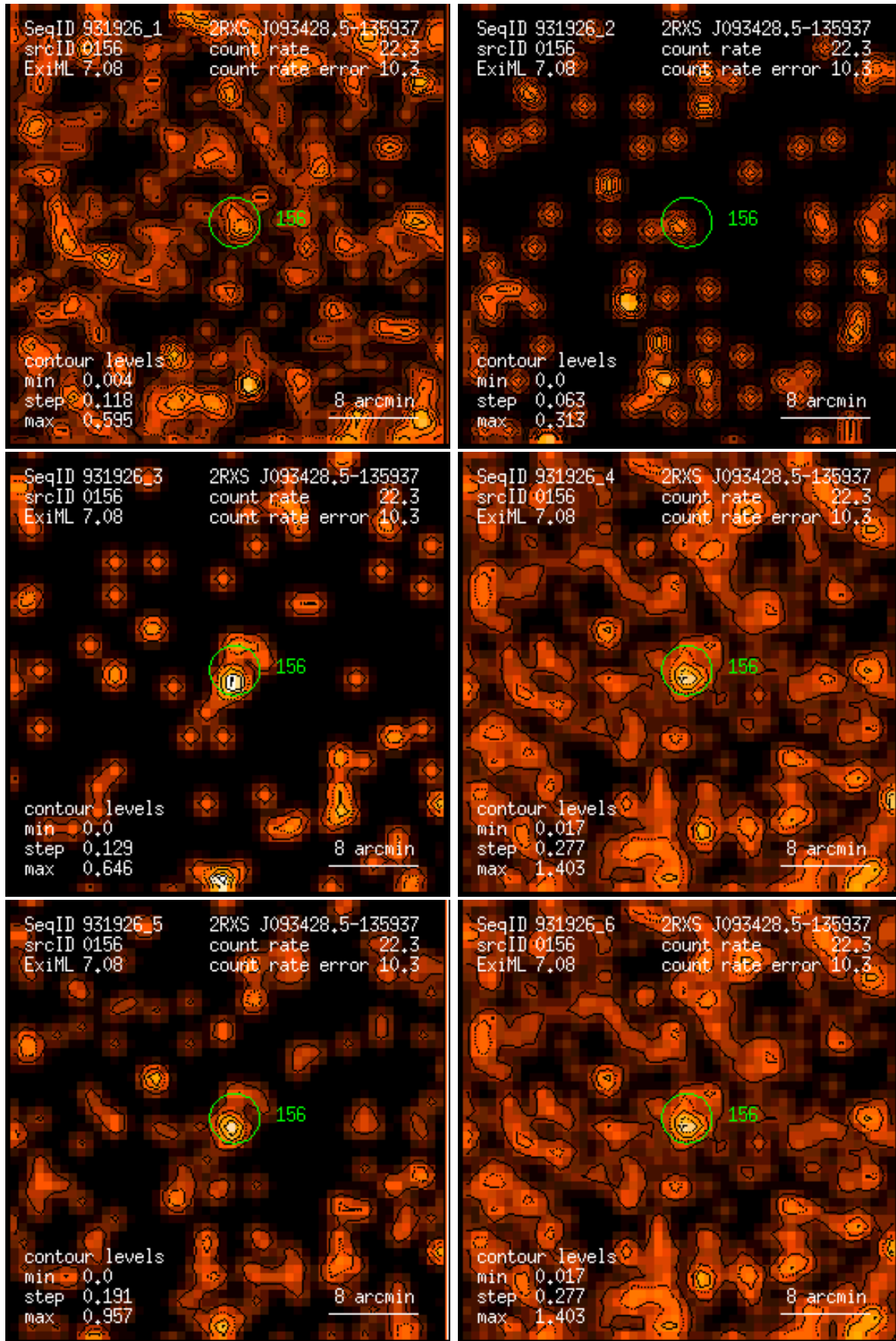
Figure 156: RASS 931926: detection 0156: band rate images, Gaussian filter: (1) PSPC channels 11 – 41, (2) 52 – 90, (3) 91 – 201, (4) 11 – 235, (5) 52 – 201, (6) 11 – 201. Broad band rates in counts/ks. Band rate contour levels in counts/ks/arcmin 2 .
