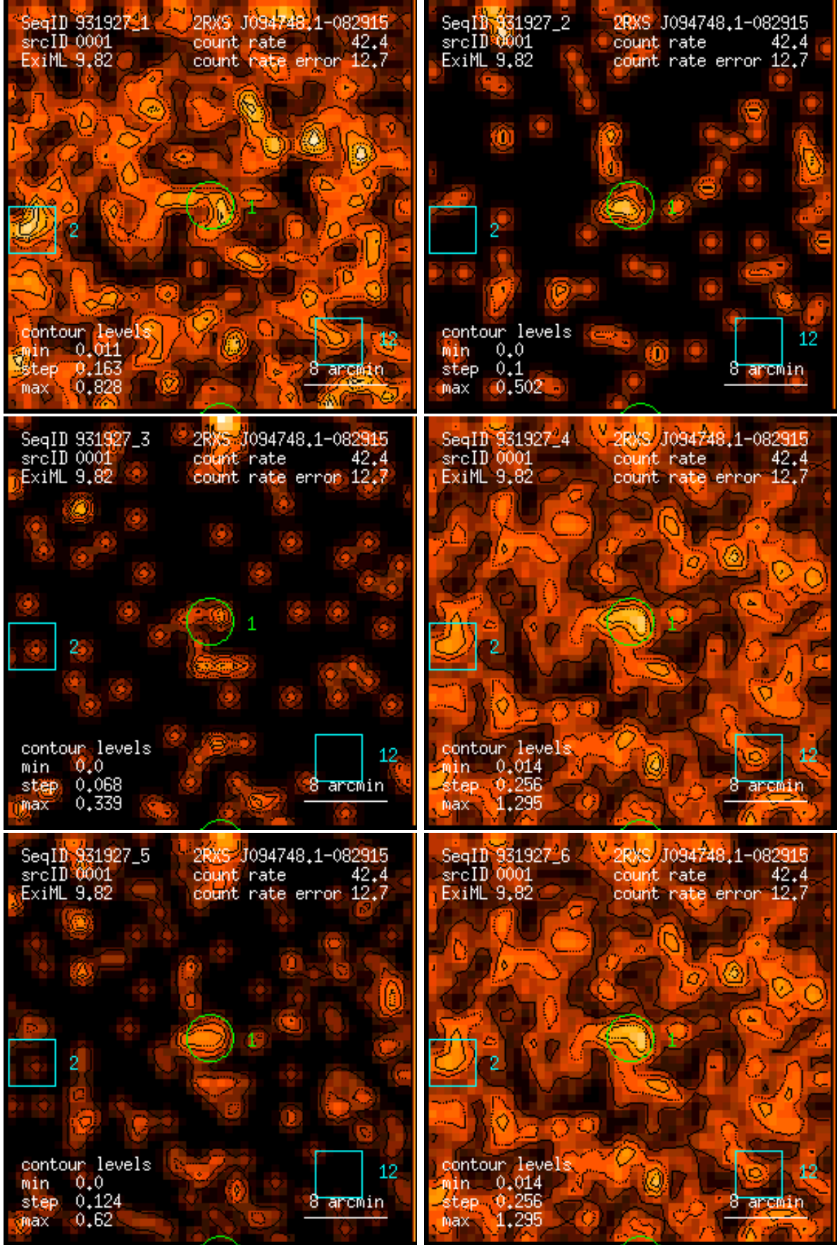
Figure 1: RASS 931927: detection 0001: band rate images, Gaussian filter: (1) PSPC channels 11 – 41, (2) 52 – 90, (3) 91 – 201, (4) 11 – 235, (5) 52 – 201, (6) 11 – 201. Broad band rates in counts/ks. Band rate contour levels in counts/ks/arcmin 2 .
