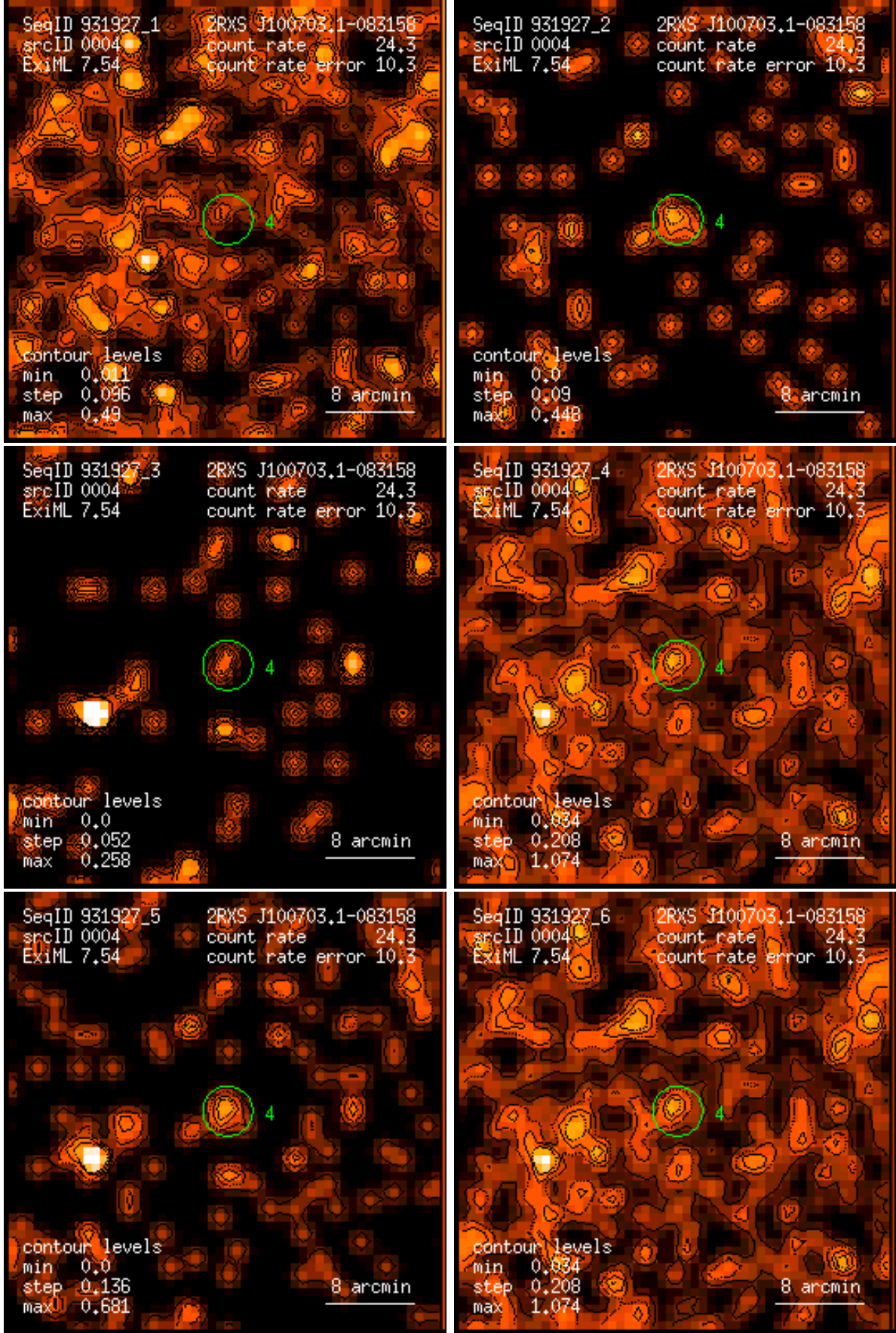
Figure 4: RASS 931927: detection 0004: band rate images, Gaussian filter: (1) PSPC channels 11 – 41, (2) 52 – 90, (3) 91 – 201, (4) 11 – 235, (5) 52 – 201, (6) 11 – 201. Broad band rates in counts/ks. Band rate contour levels in counts/ks/arcmin 2 .
