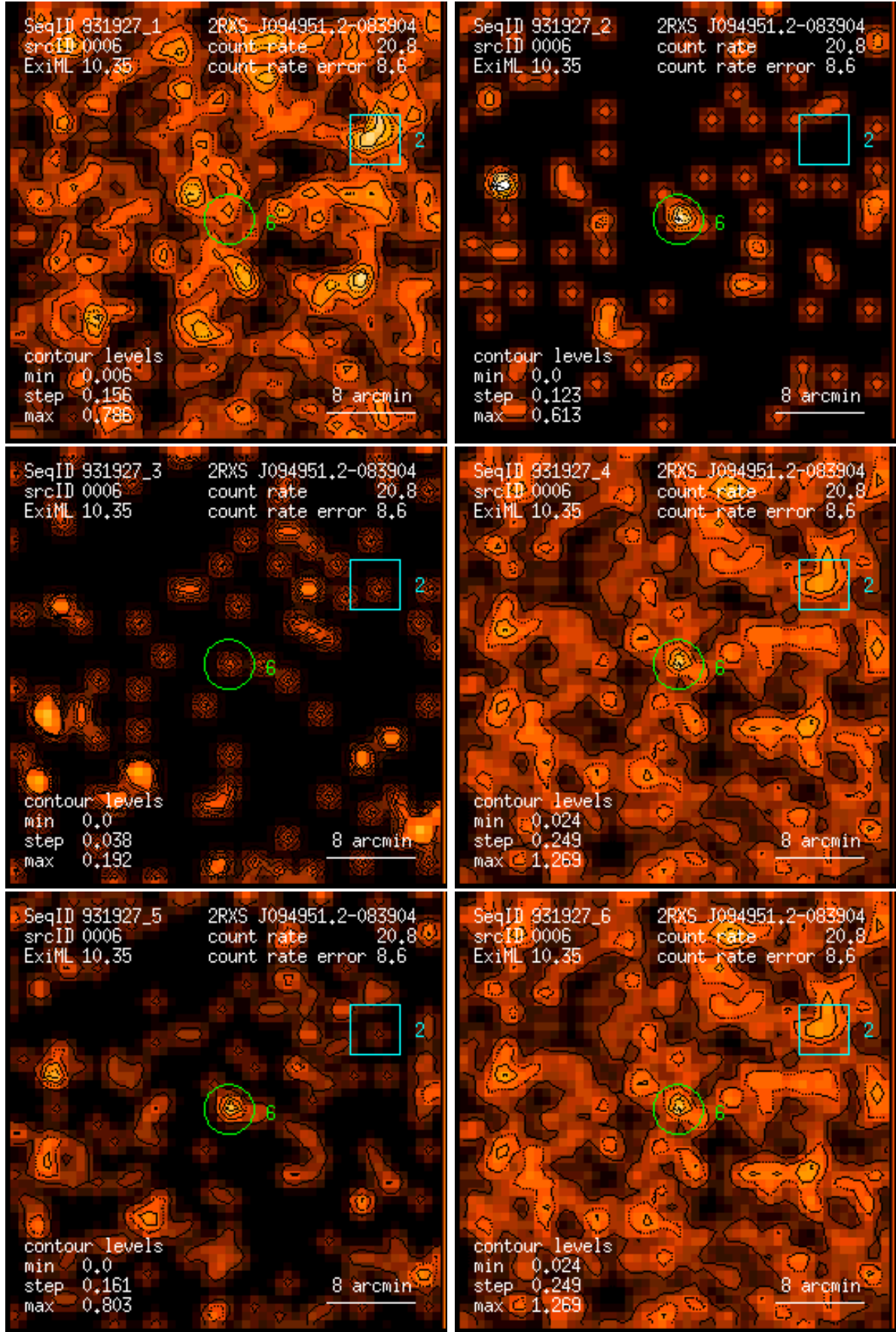
Figure 6: RASS 931927: detection 0006: band rate images, Gaussian filter: (1) PSPC channels 11 – 41, (2) 52 – 90, (3) 91 – 201, (4) 11 – 235, (5) 52 – 201, (6) 11 – 201. Broad band rates in counts/ks. Band rate contour levels in counts/ks/arcmin 2 .
