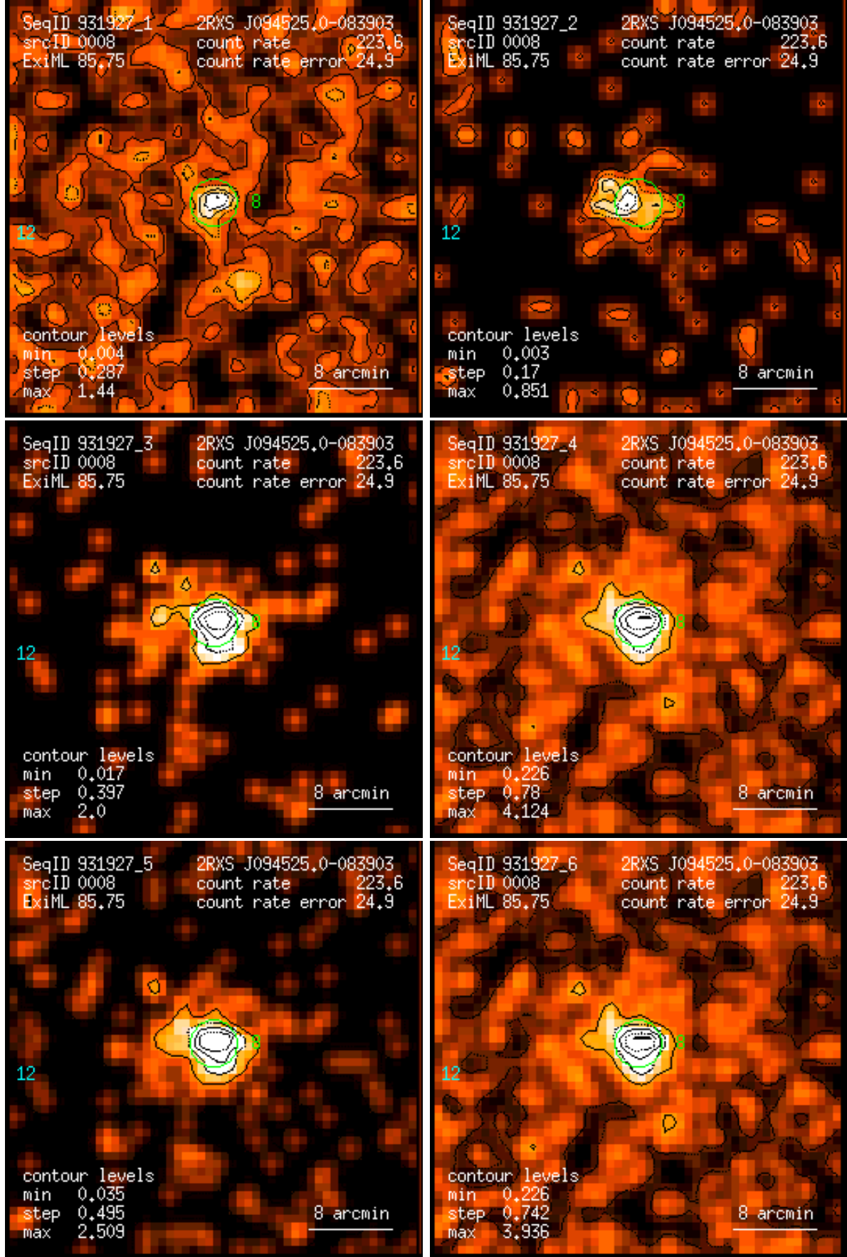
Figure 8: RASS 931927: detection 0008: band rate images, Gaussian filter: (1) PSPC channels 11 – 41, (2) 52 – 90, (3) 91 – 201, (4) 11 – 235, (5) 52 – 201, (6) 11 – 201. Broad band rates in counts/ks. Band rate contour levels in counts/ks/arcmin 2 .
