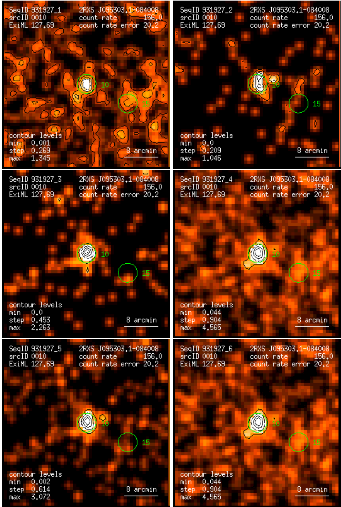
Figure 10: RASS 931927: detection 0010: band rate images, Gaussian filter: (1) PSPC channels 11 – 41, (2) 52 – 90, (3) 91 – 201, (4) 11 – 235, (5) 52 – 201, (6) 11 – 201. Broad band rates in counts/ks. Band rate contour levels in counts/ks/arcmin 2 .
