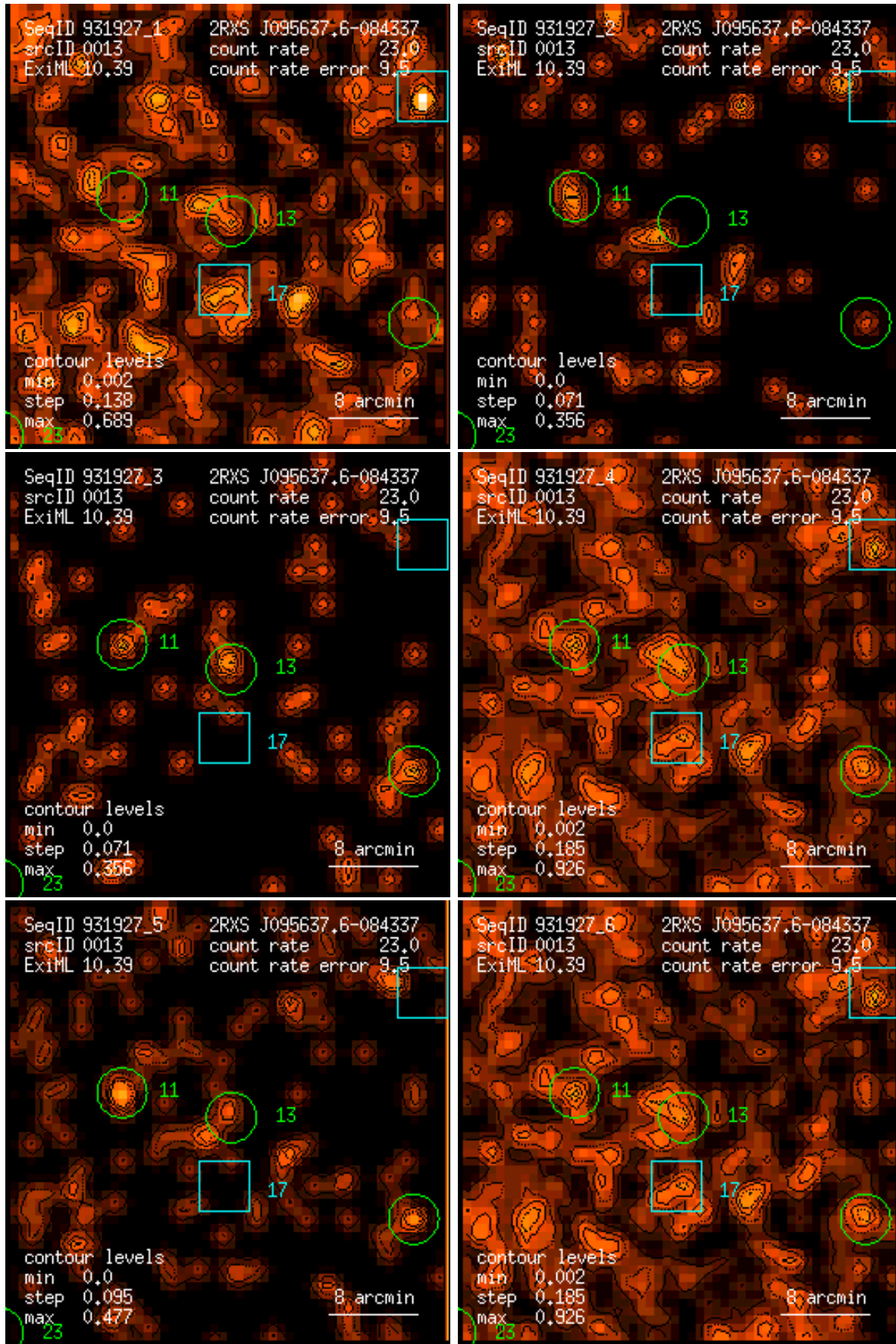
Figure 13: RASS 931927: detection 0013: band rate images, Gaussian filter: (1) PSPC channels 11 – 41, (2) 52 – 90, (3) 91 – 201, (4) 11 – 235, (5) 52 – 201, (6) 11 – 201. Broad band rates in counts/ks. Band rate contour levels in counts/ks/arcmin 2 .
