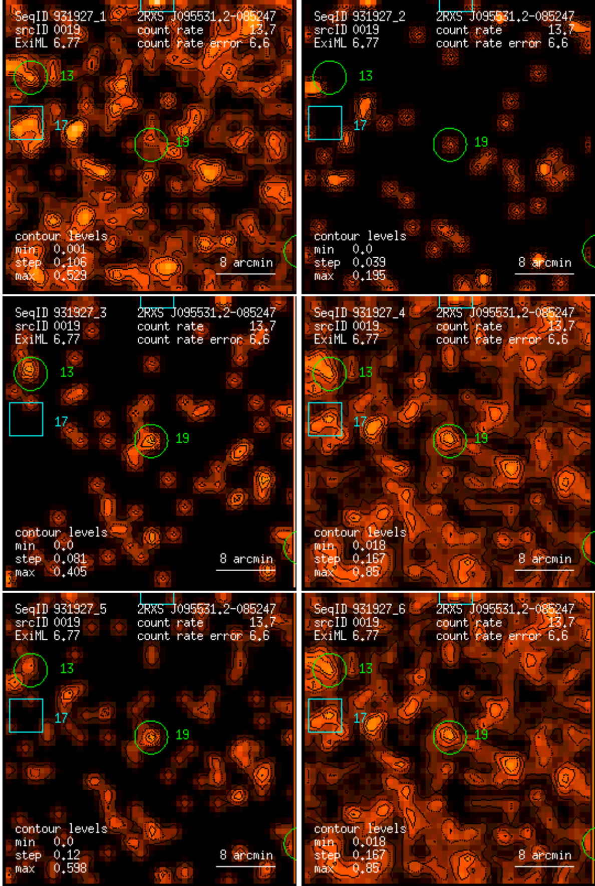
Figure 19: RASS 931927: detection 0019: band rate images, Gaussian filter: (1) PSPC channels 11 – 41, (2) 52 – 90, (3) 91 – 201, (4) 11 – 235, (5) 52 – 201, (6) 11 – 201. Broad band rates in counts/ks. Band rate contour levels in counts/ks/arcmin 2 .
