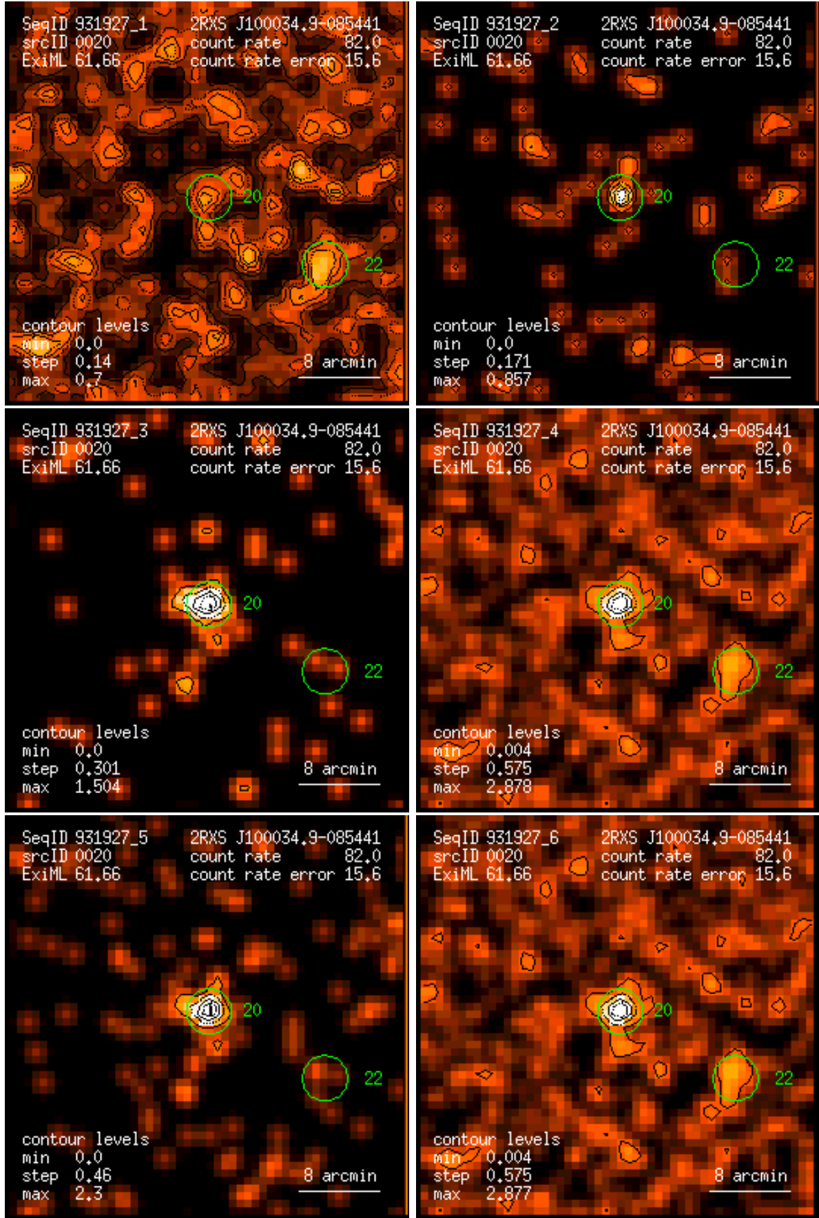
Figure 20: RASS 931927: detection 0020: band rate images, Gaussian filter: (1) PSPC channels 11 – 41, (2) 52 – 90, (3) 91 – 201, (4) 11 – 235, (5) 52 – 201, (6) 11 – 201. Broad band rates in counts/ks. Band rate contour levels in counts/ks/arcmin 2 .
