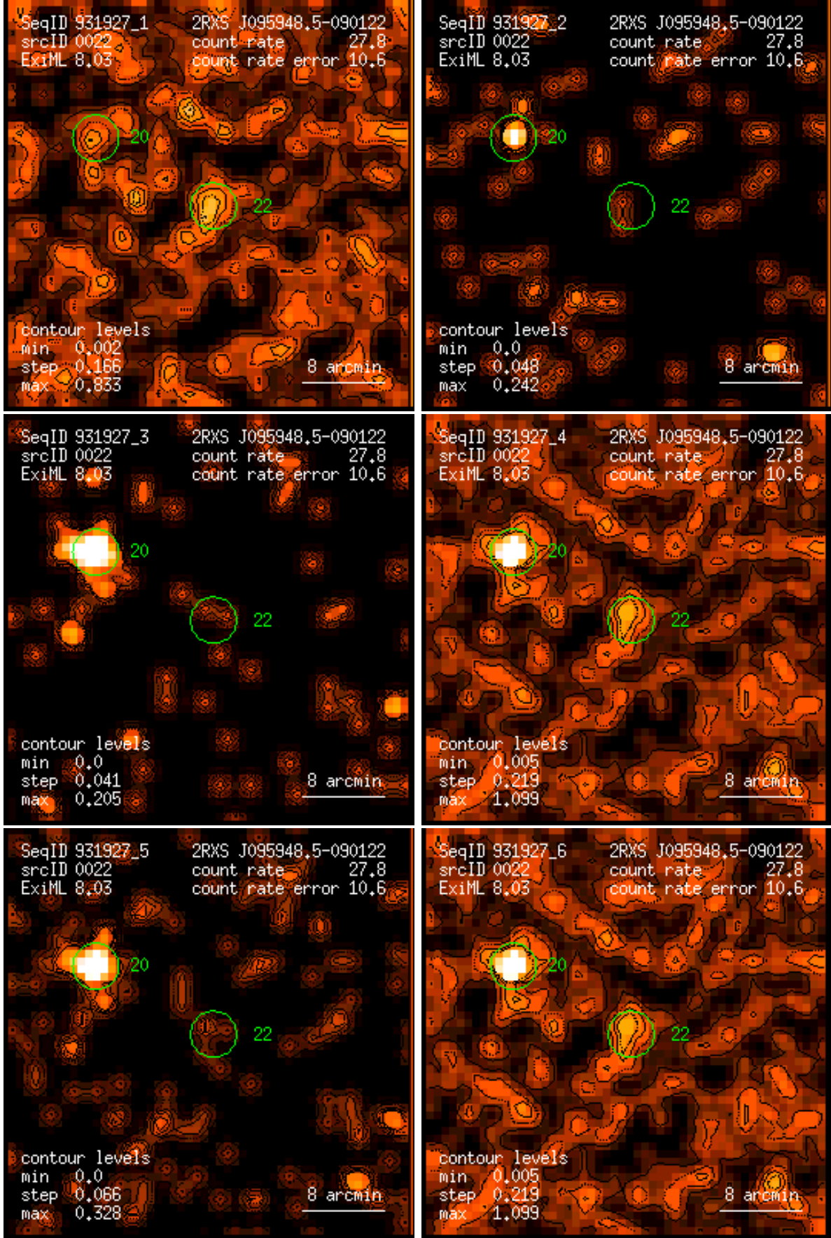
Figure 22: RASS 931927: detection 0022: band rate images, Gaussian filter: (1) PSPC channels 11 – 41, (2) 52 – 90, (3) 91 – 201, (4) 11 – 235, (5) 52 – 201, (6) 11 – 201. Broad band rates in counts/ks. Band rate contour levels in counts/ks/arcmin 2 .
