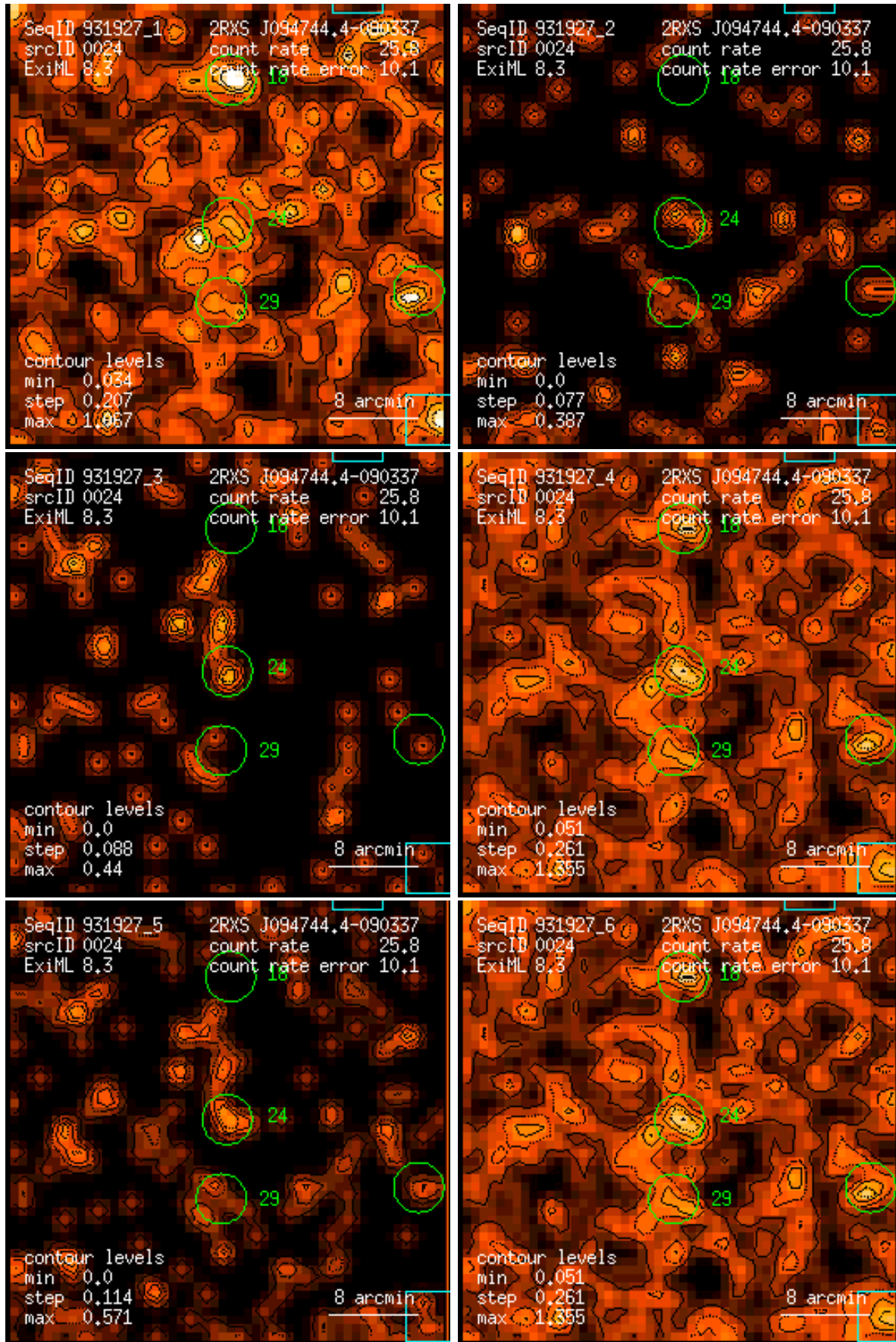
Figure 24: RASS 931927: detection 0024: band rate images, Gaussian filter: (1) PSPC channels 11 – 41, (2) 52 – 90, (3) 91 – 201, (4) 11 – 235, (5) 52 – 201, (6) 11 – 201. Broad band rates in counts/ks. Band rate contour levels in counts/ks/arcmin 2 .
