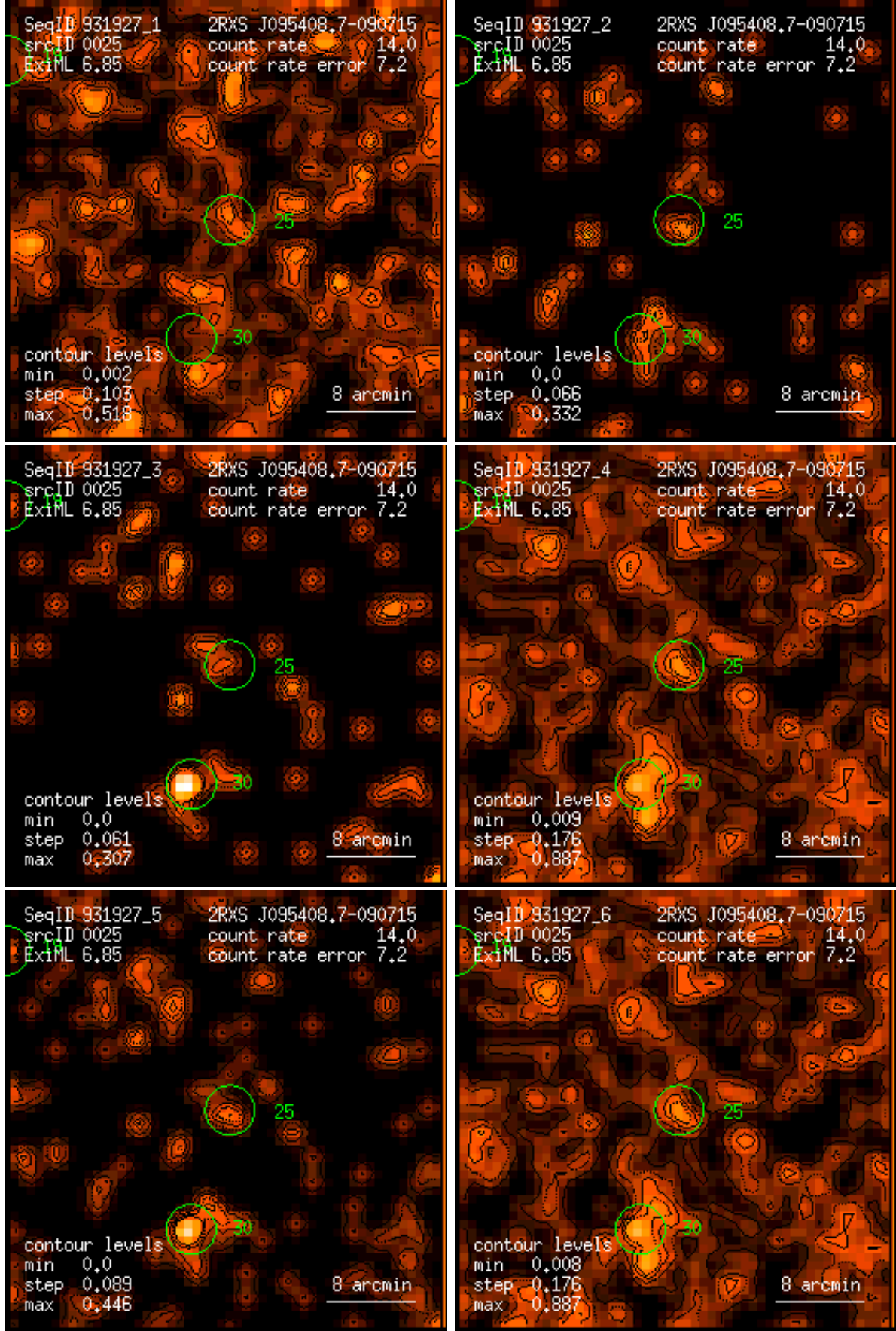
Figure 25: RASS 931927: detection 0025: band rate images, Gaussian filter: (1) PSPC channels 11 – 41, (2) 52 – 90, (3) 91 – 201, (4) 11 – 235, (5) 52 – 201, (6) 11 – 201. Broad band rates in counts/ks. Band rate contour levels in counts/ks/arcmin 2 .
